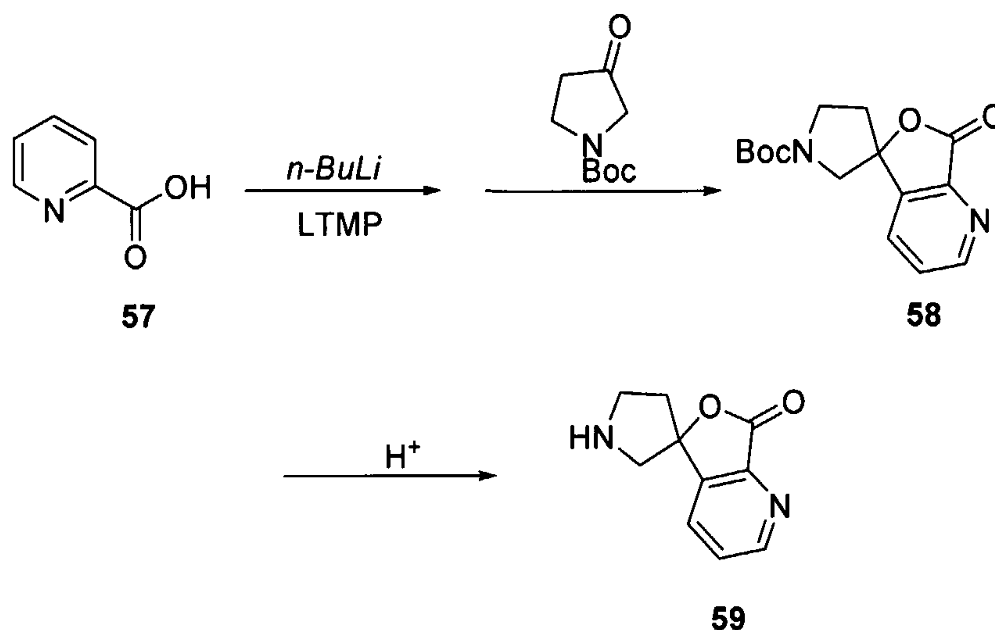
Scheme 15
