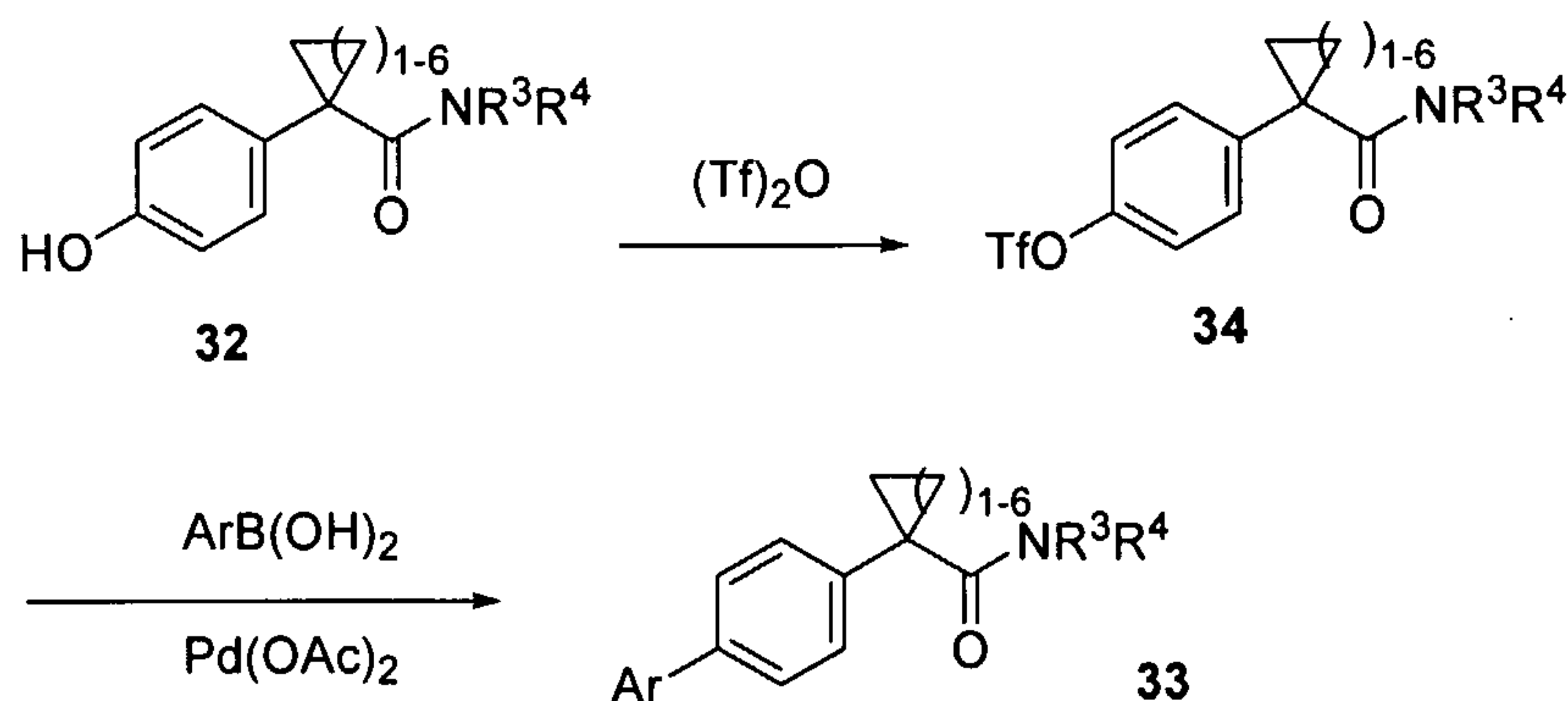
Scheme 11
