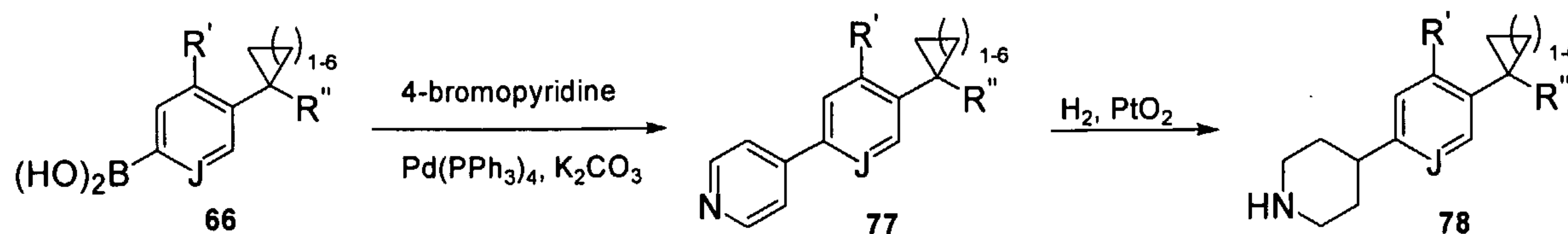
Scheme 20
