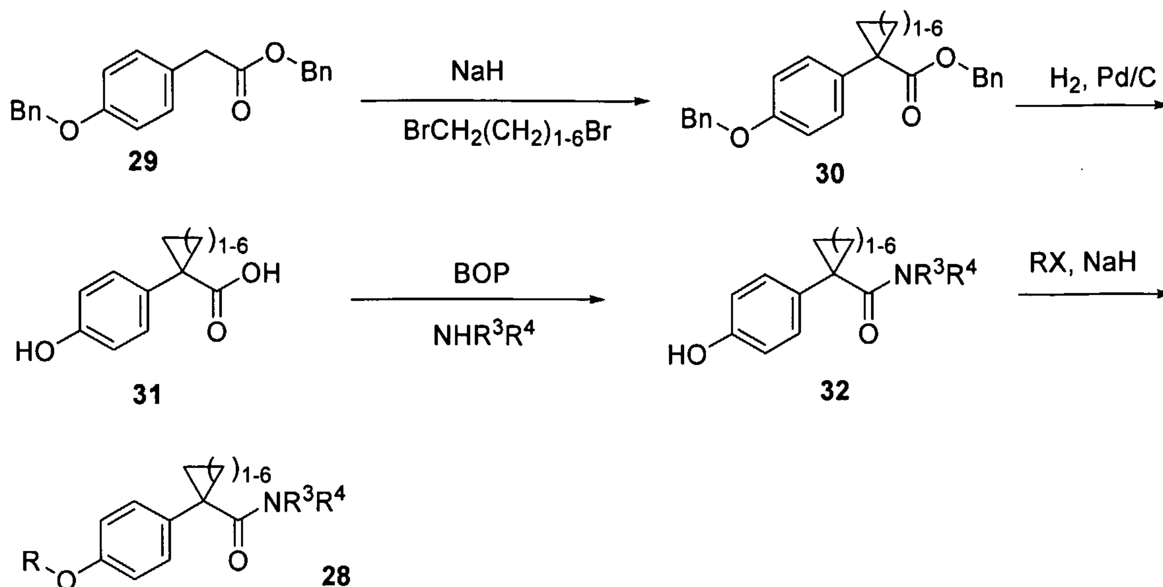
Scheme 10
