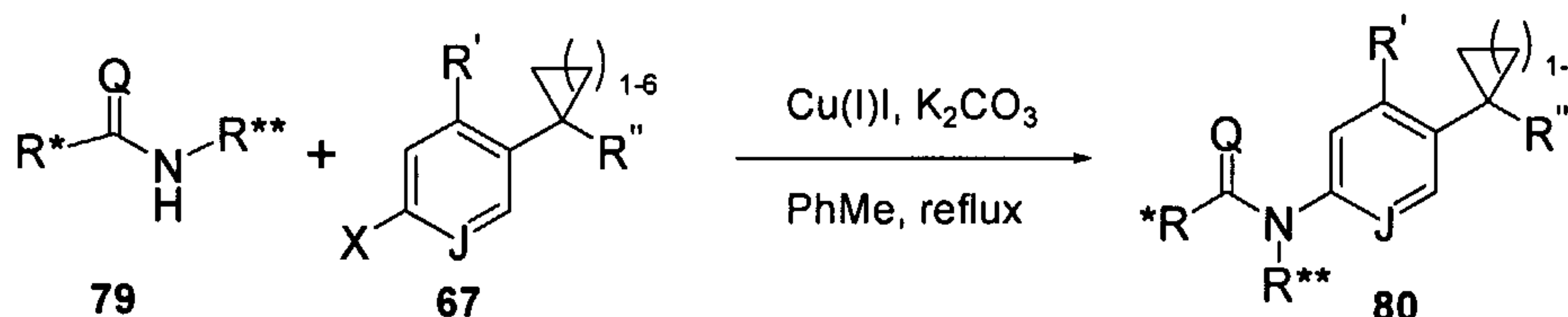
Scheme 21
