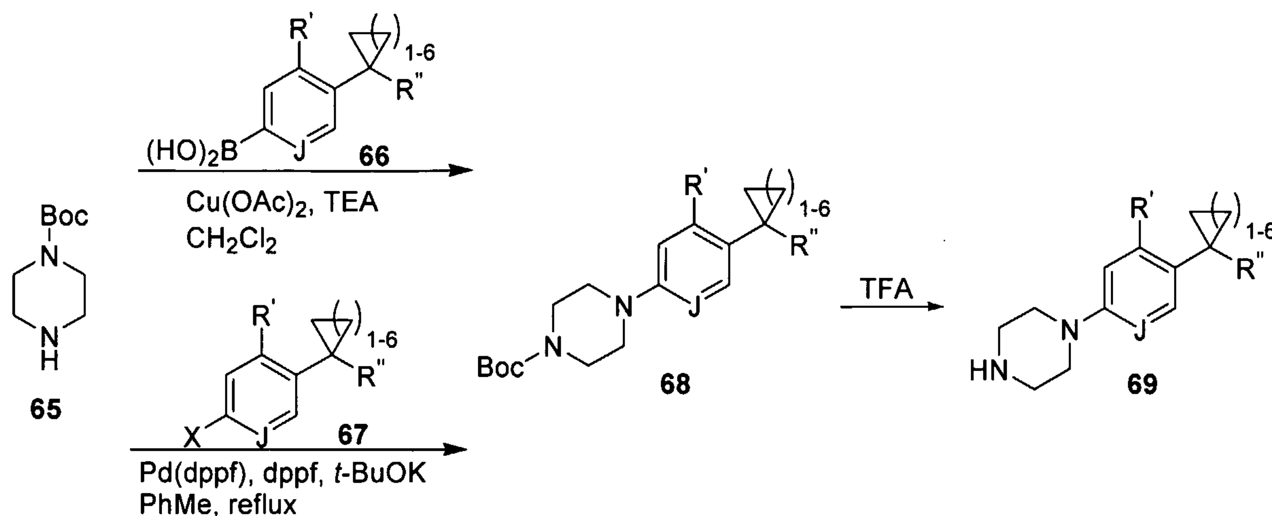
Scheme 17
