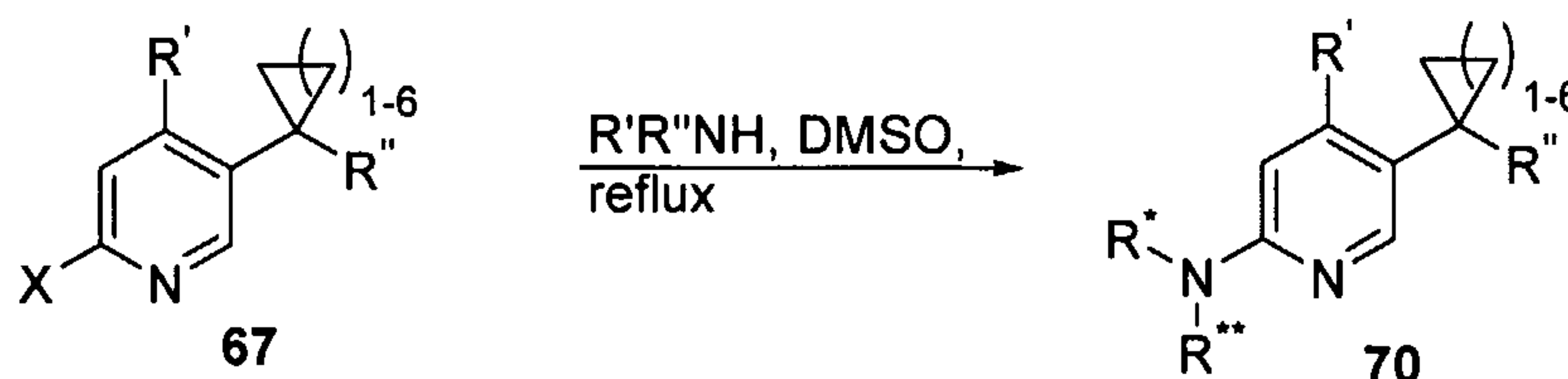
Scheme 18
