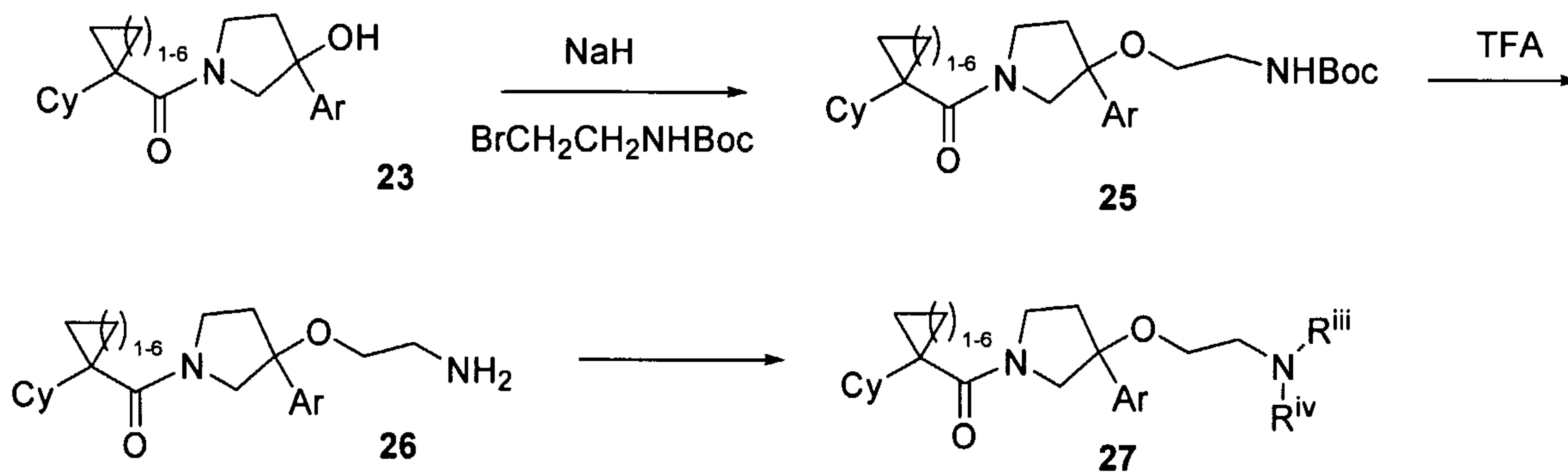
Scheme 9
