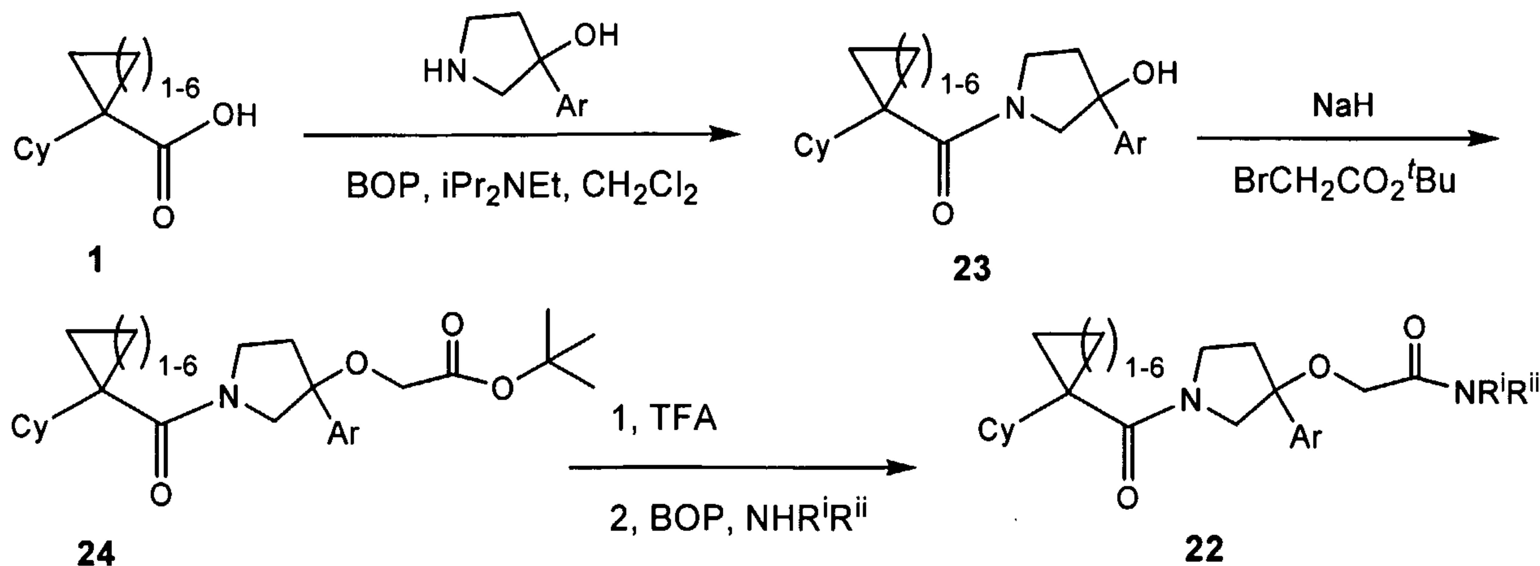
Scheme 8
