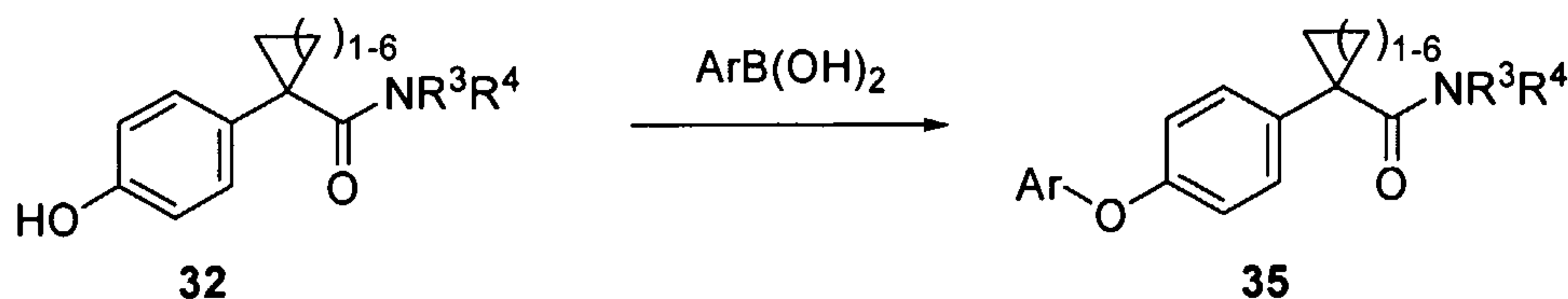
Scheme 12
