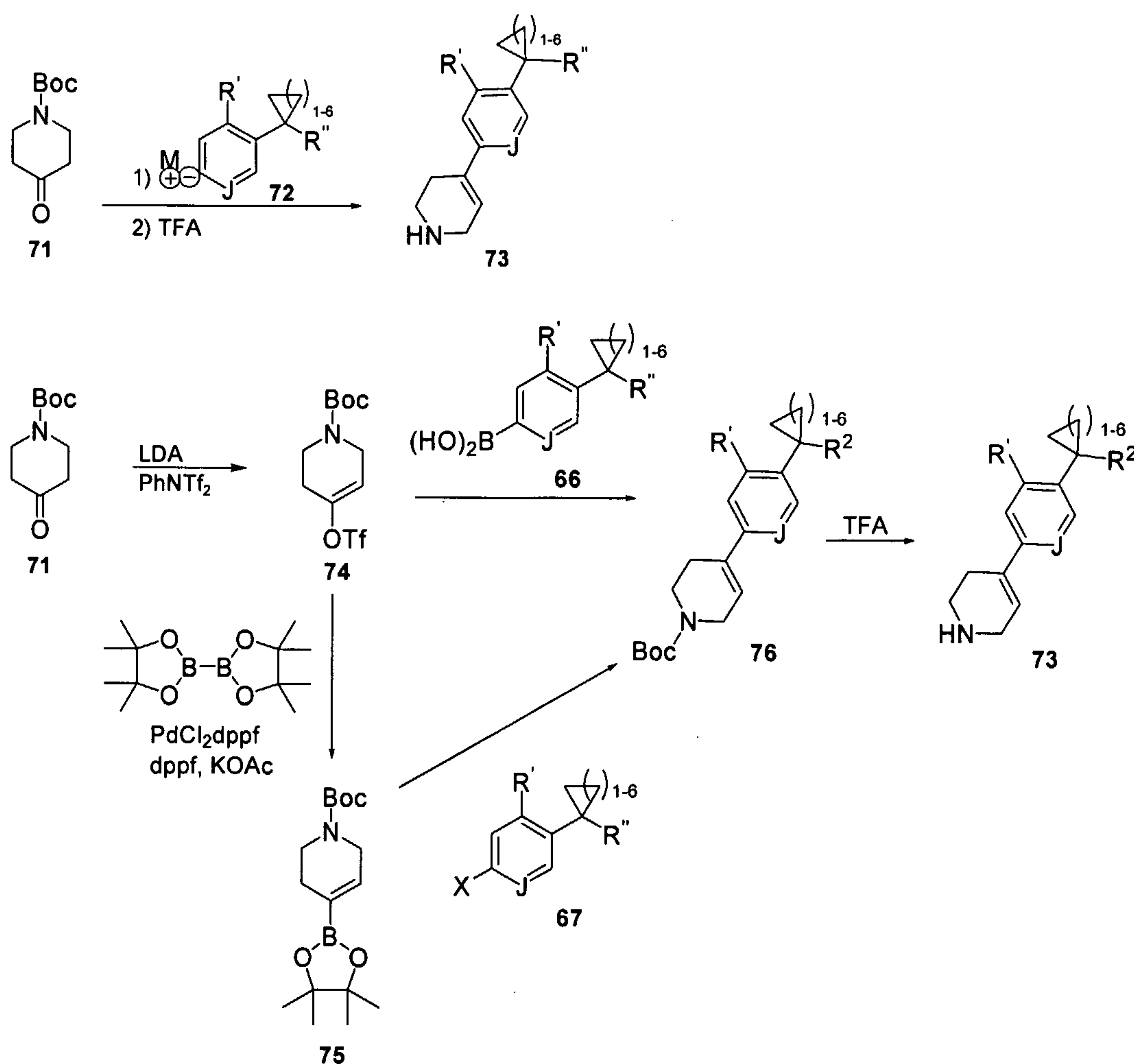
Scheme 19
