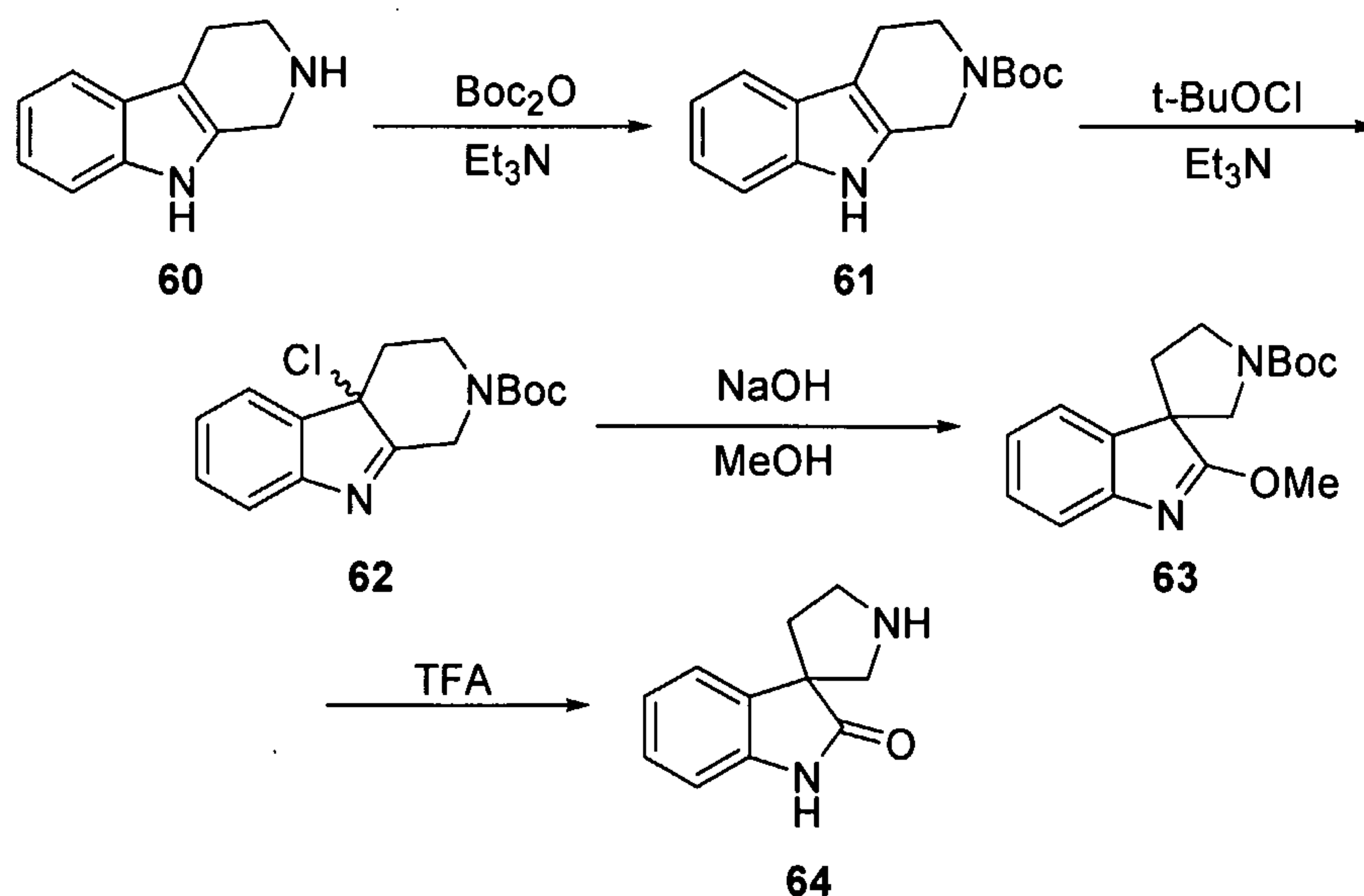
Scheme 16
