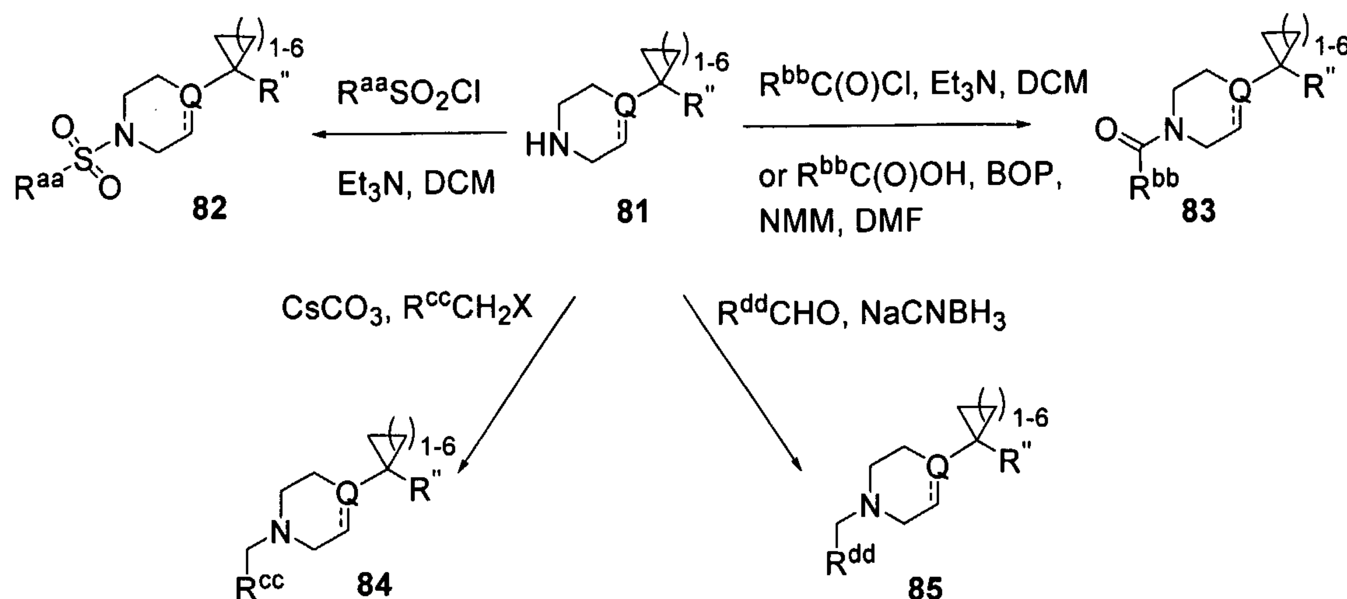
Scheme 22
