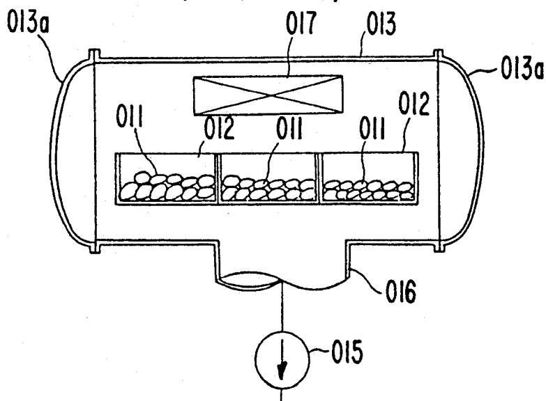
FIG. 19 (PRIOR ART)
