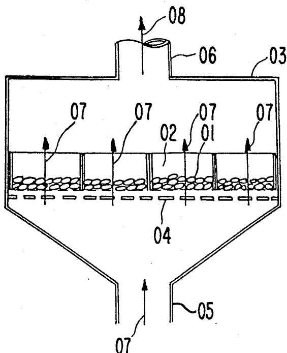
FIG. 18 (PRIOR ART)
