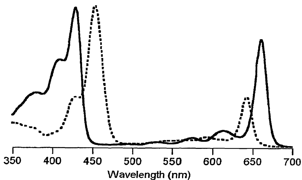
Figure 3. Absorption spectra of chlorophylls a and b.
