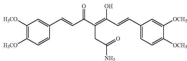
Compound JM2
