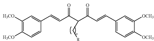
Compound Q49: n = 1 , R = \text{CON}(\text{C}_2\text{H}_5)_2
