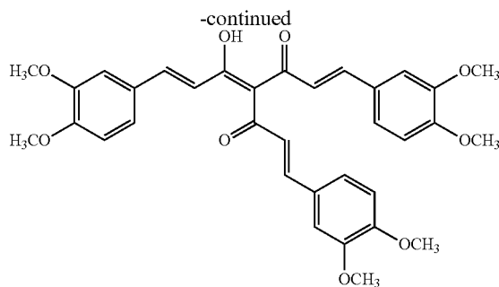
compound JM4
