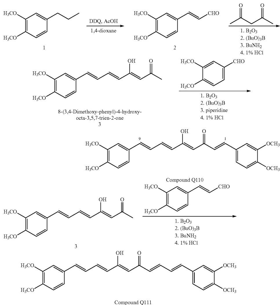
Scheme 13
