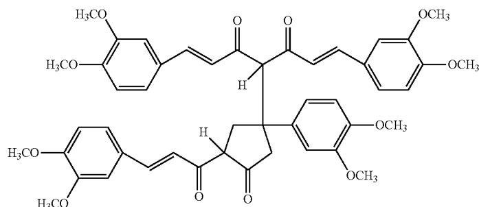
compound JM5
