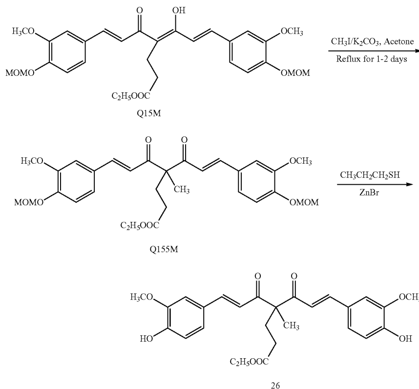
Scheme 18
