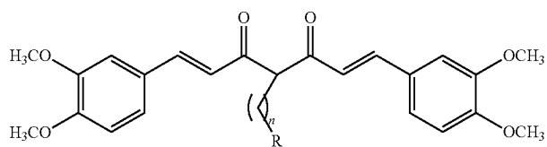
Compound Q44: n = 1 , R = \text{COOC}_2\text{H}_5
