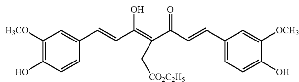
Compound Q50
