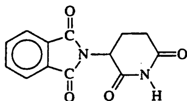
thalidomide
