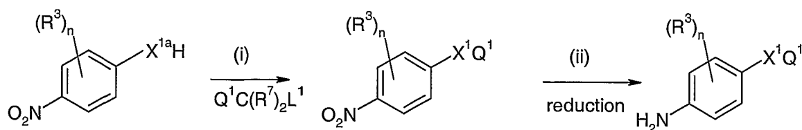
Reaction Scheme 3
