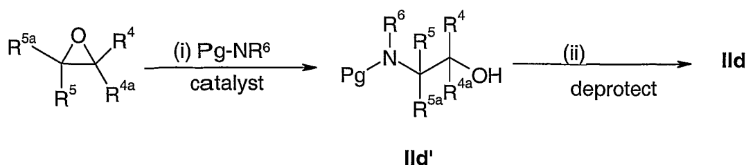
Reaction Scheme 4
