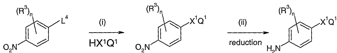
Reaction Scheme 2
