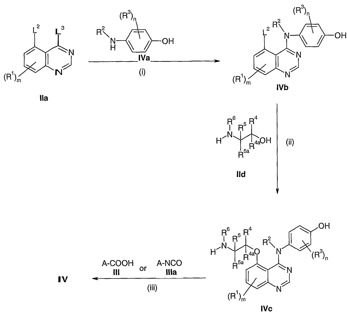
Reaction Scheme 5
