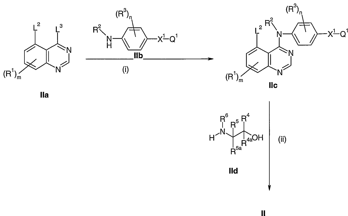
Reaction Scheme 1
