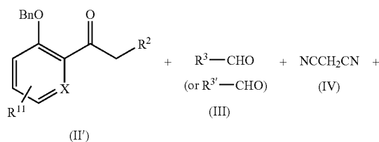
Reaction A
