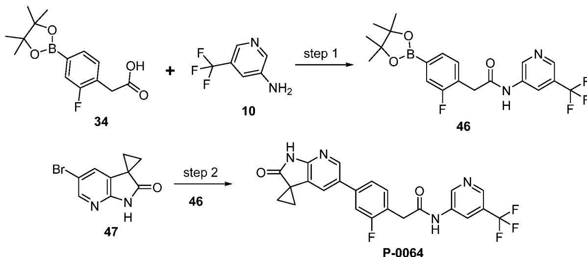
Scheme 12
