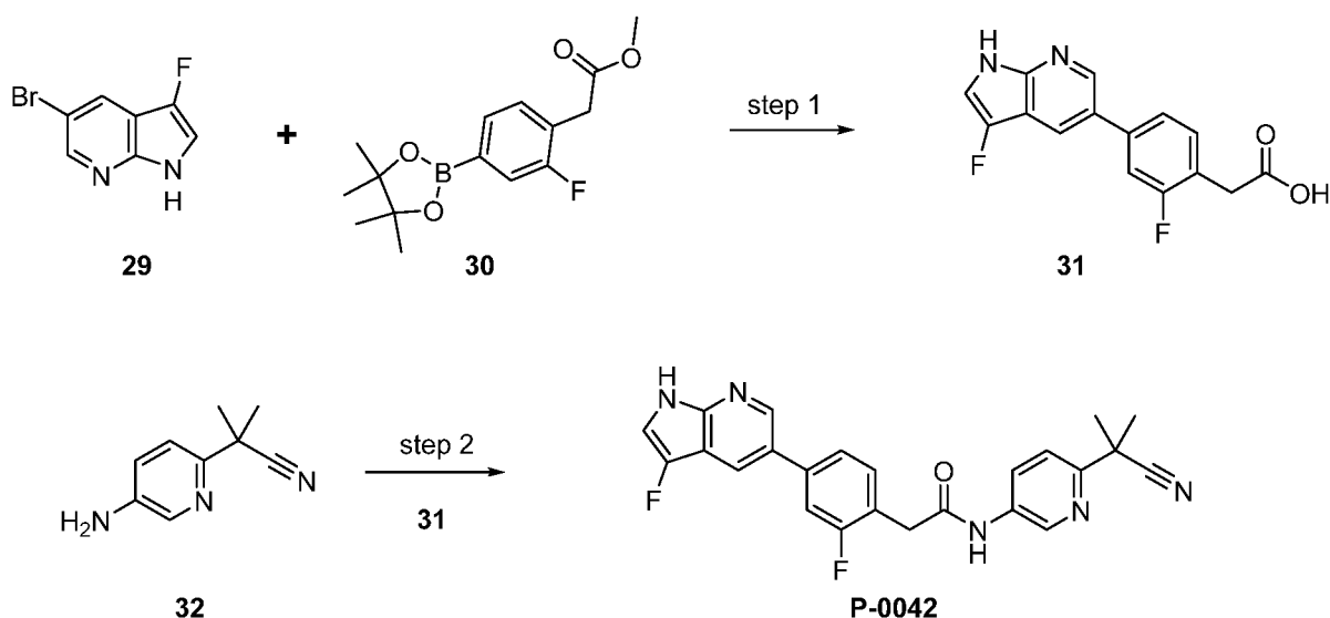
Scheme 7
