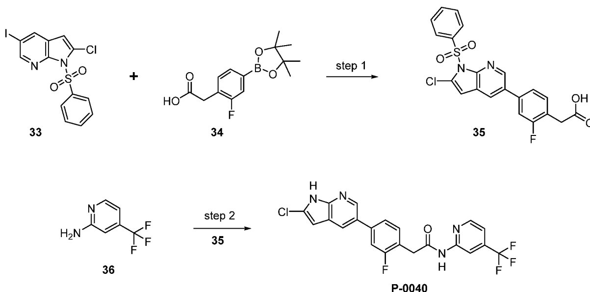
Scheme 8
