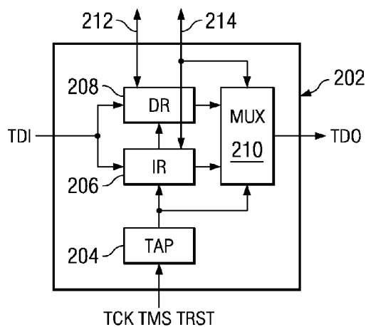
FIG. 2 (PRIOR ART)
