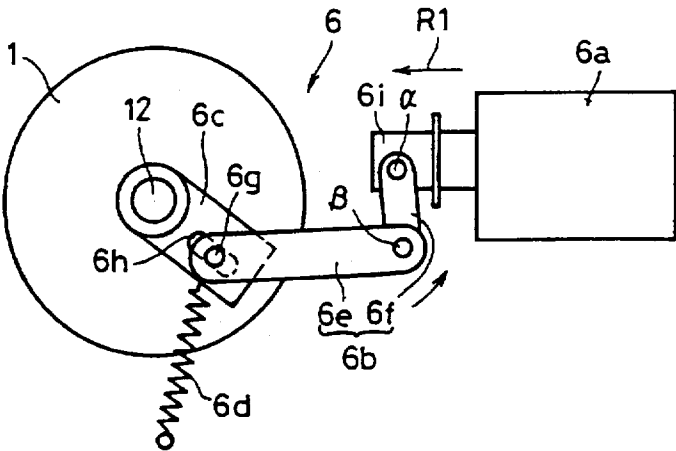
FIG. 4B NEUTRAL-STATE OF SOLENOID
