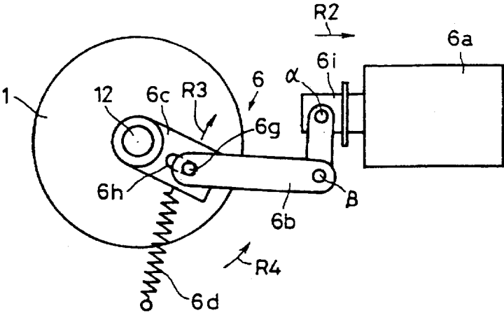
FIG. 4B NEUTRAL-STATE OF SOLENOID
