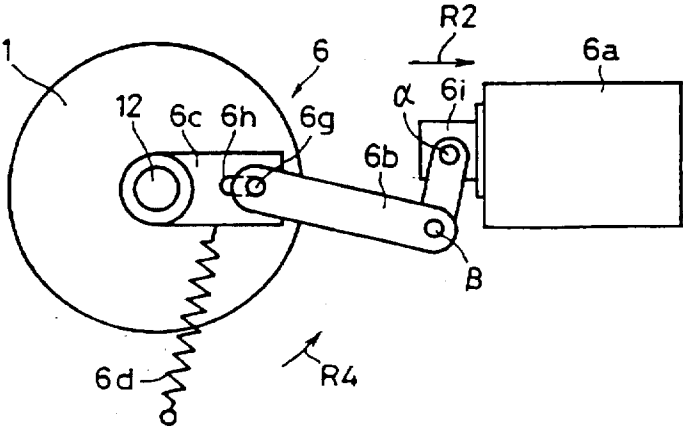
FIG. 4C ON-STATE OF SOLENOID
