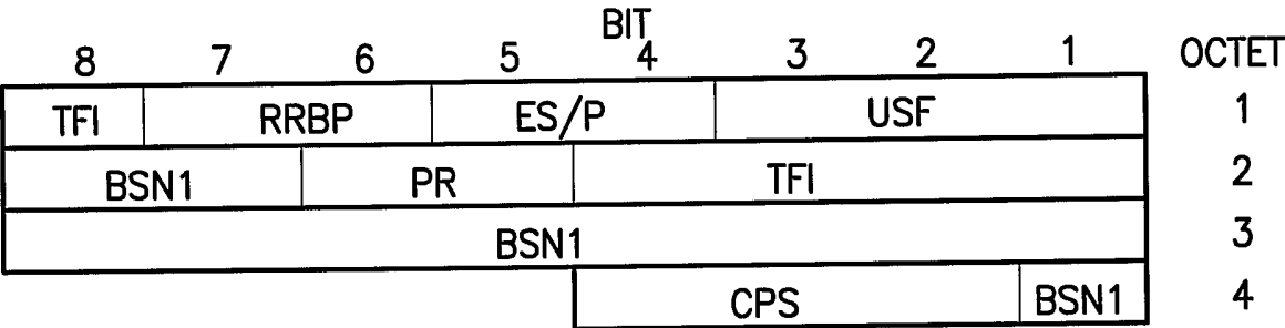
EGPRS DOWNLINK RLC DATA BLOCK HEADER FOR MCS-5 AND MCS-6
