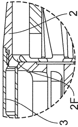
DETAIL C SCALE 2:1 FIG. 3D
