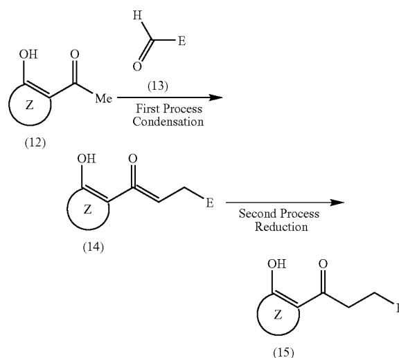
Reaction Scheme 4
