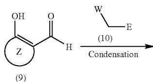
Reaction Scheme 3
