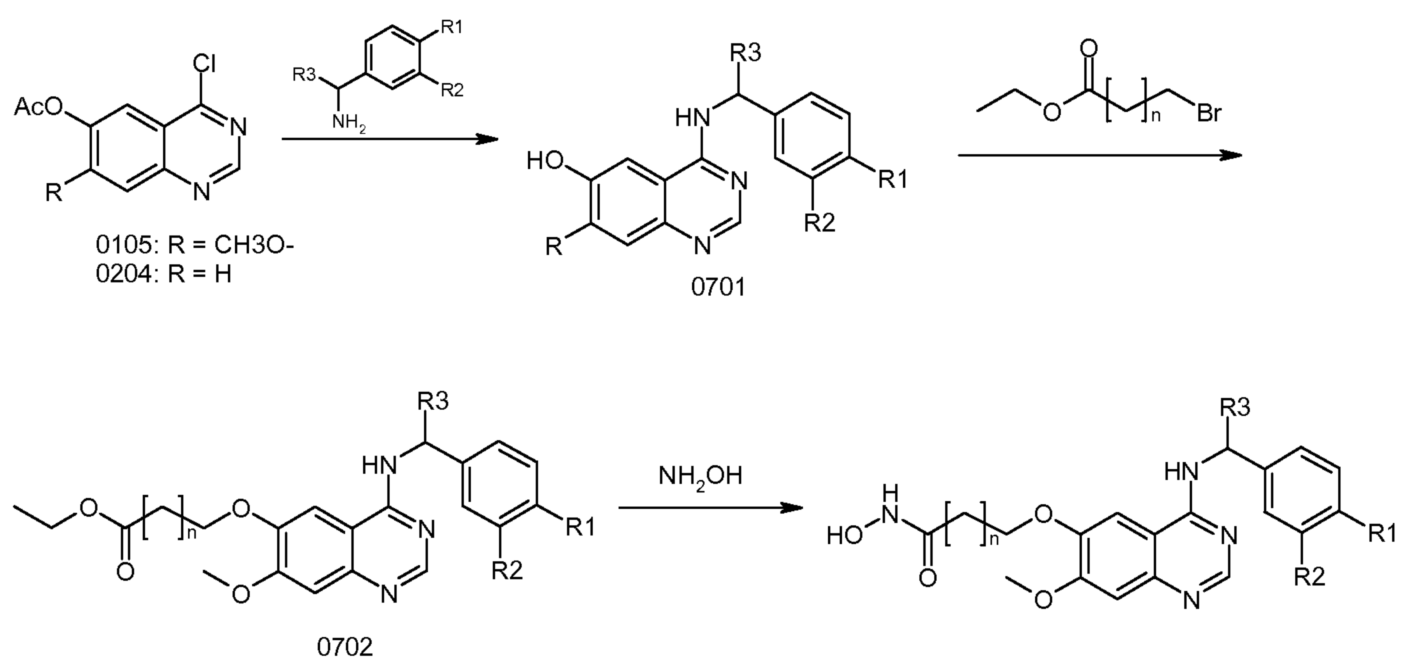
Scheme 7
