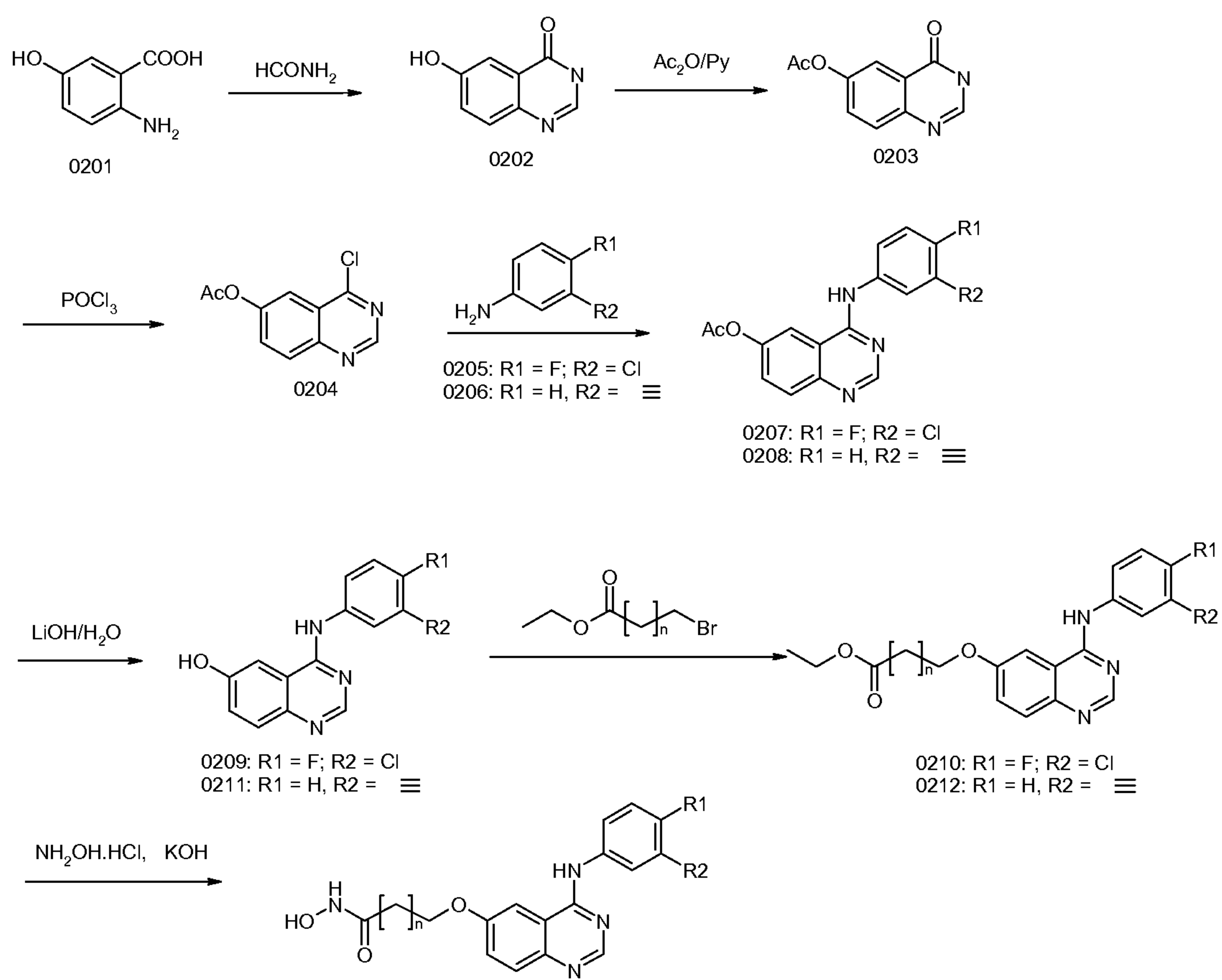
Scheme 2
