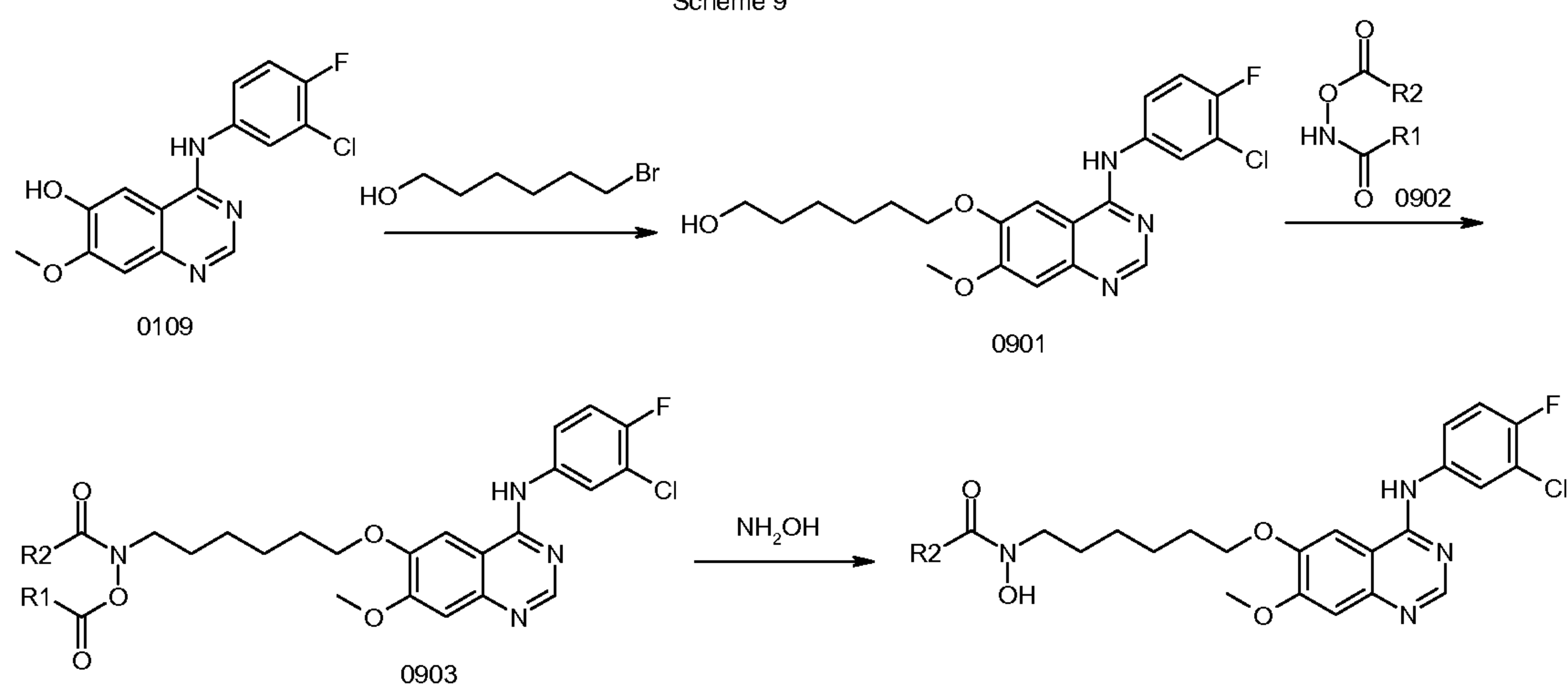
Scheme 9
