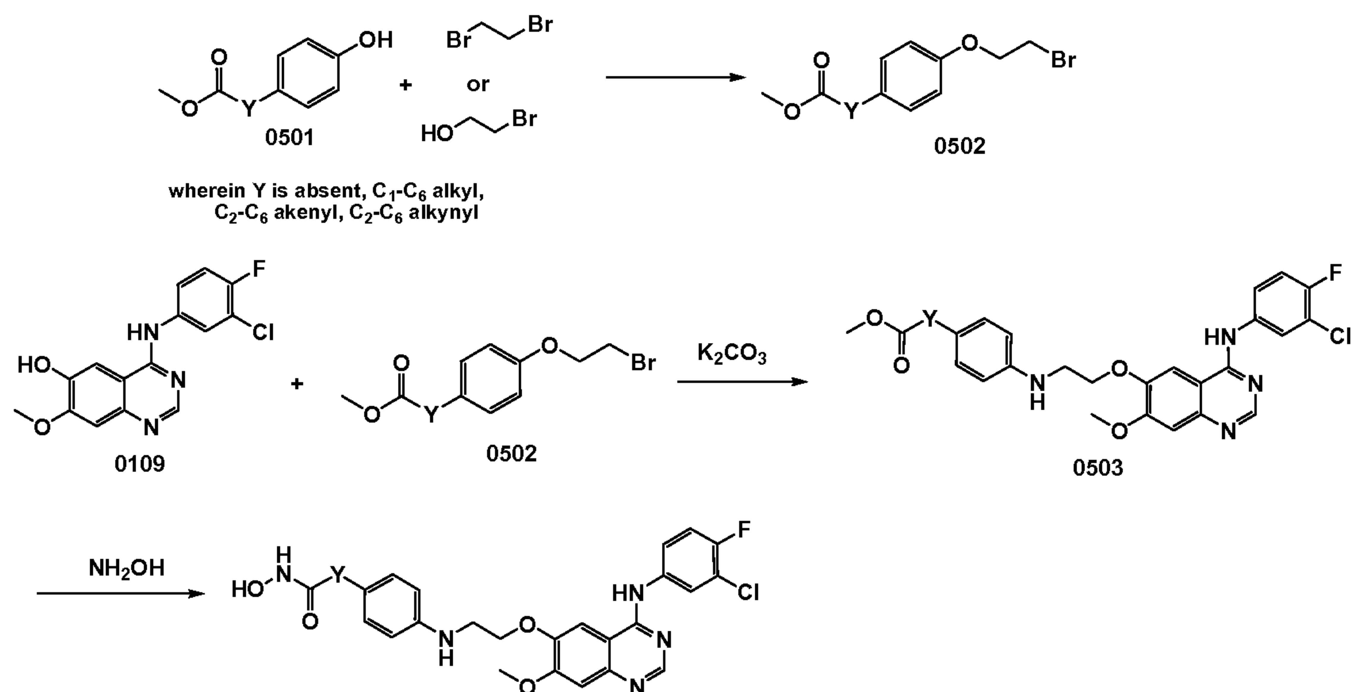
Scheme 5
