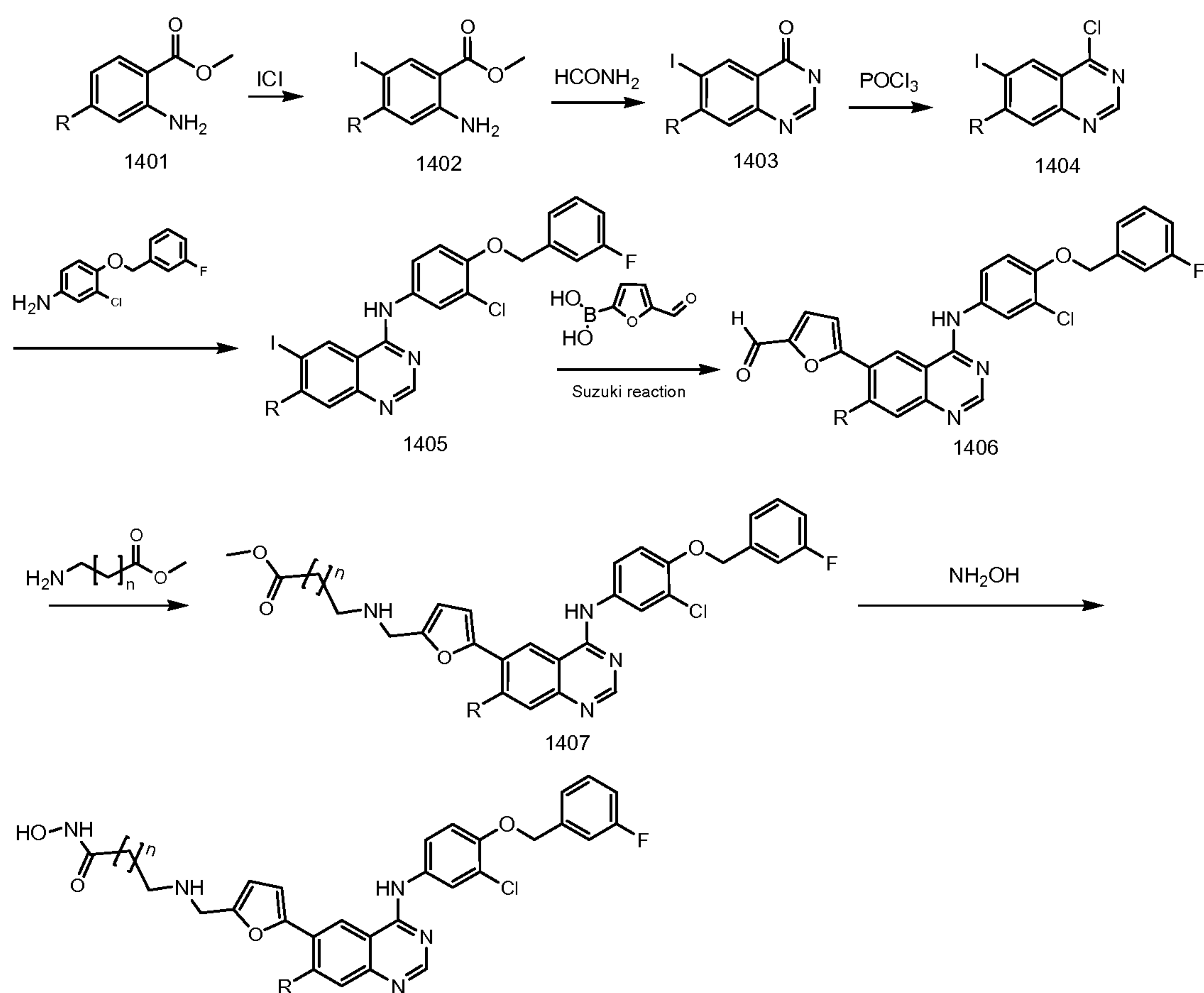
Scheme 14
