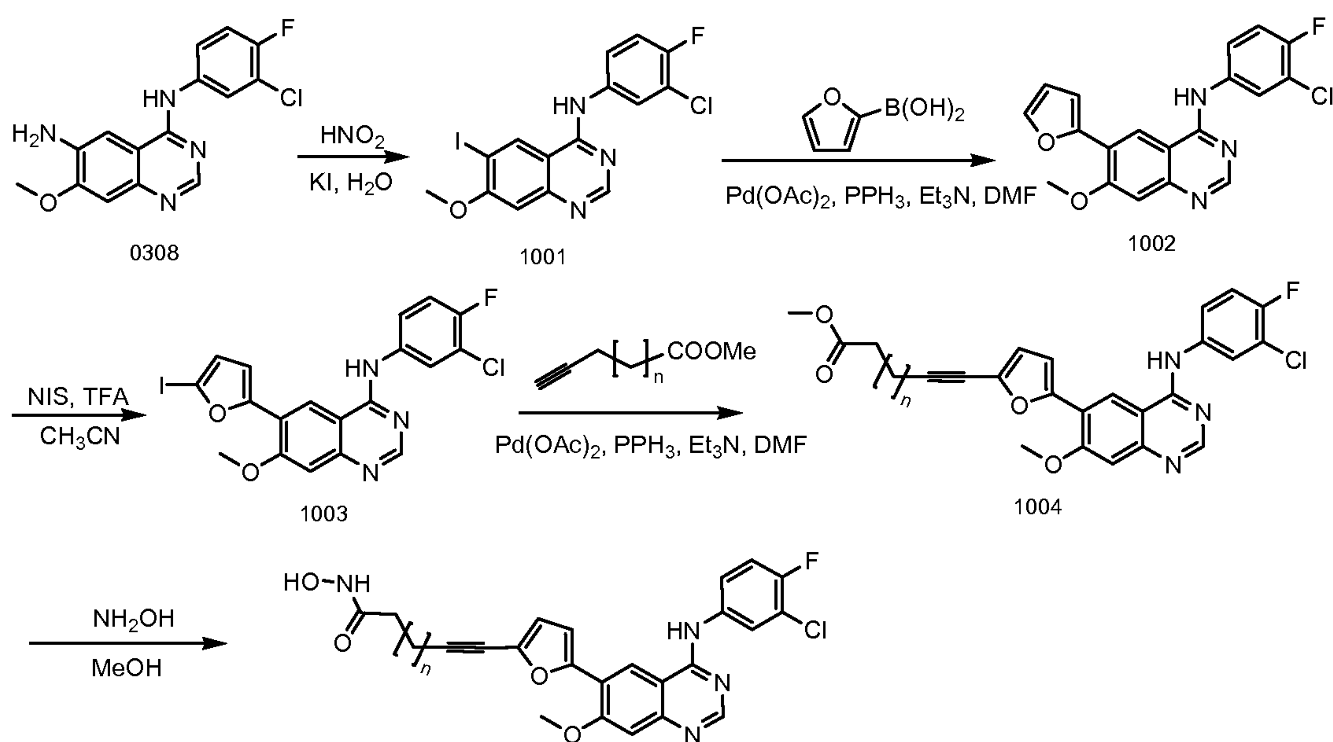
Scheme 10
