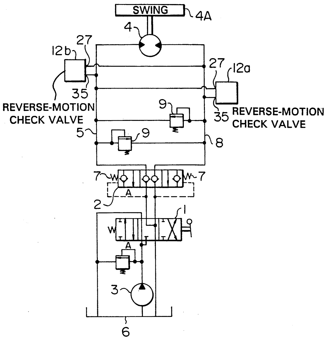
FIG. 3 PRIOR ART
