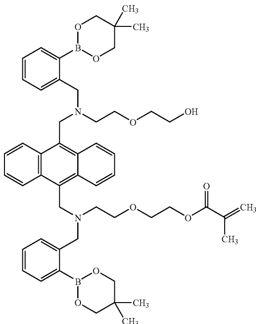
C. 9-[N-[2-(5,5-dimethyl-1,3,2)dioxaborinan-2-yl)benzyl]-N-[2-(2-methacroyloxyethoxy)ethylamino]methyl]-10-[N-[2-(5,5-dimethyl-1,3,2)dioxaborinan-2-yl)benzyl]-N-[2-(2-hydroxyethoxy)ethylamino]methyl]anthracene. (Single-methacrylate monomer)
