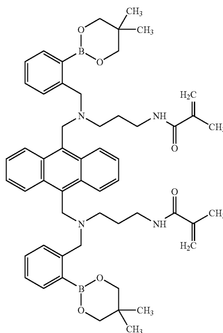
B. 9,10-bis[N-[2-(5,5-dimethyl-[1,3,2]dioxaborinan-2-yl)benzyl]-N-[3-(methacrylamido)propylamino]methylanthracene
