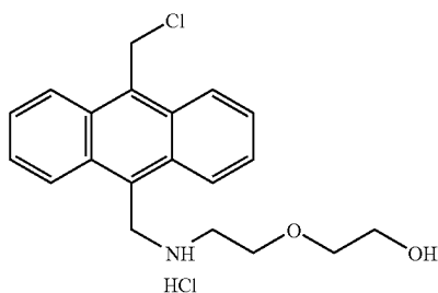
A. 9-chloromethyl-10-[[2-(2-hydroxyethoxy)ethylamino]-methyl]anthracene hydrochloride salt
