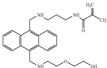
B. 9-[[2-(2-hydroxyethoxy)ethylamino]methyl]-10-[[3-(methacrylamido)propylamino]methyl]anthracene
