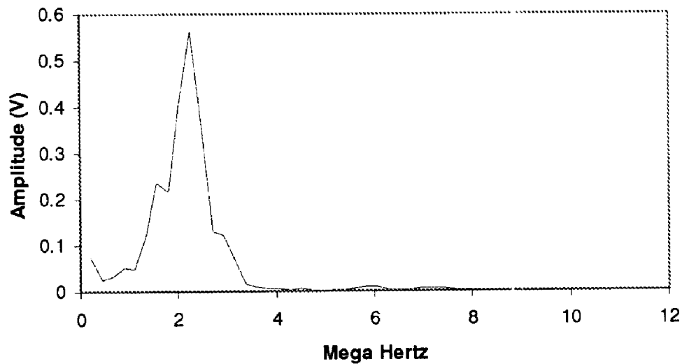
Amplitude (Volts) vs. Frequency (Mega Hertz) for Region A
