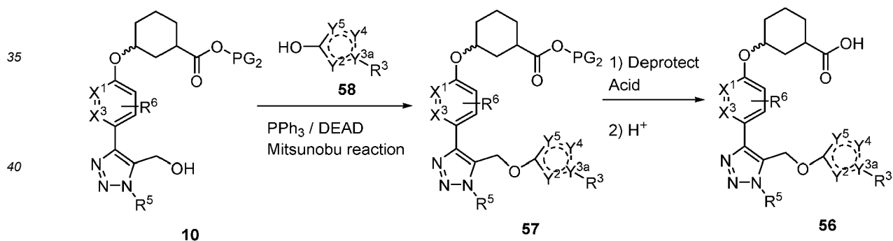
Scheme 11
