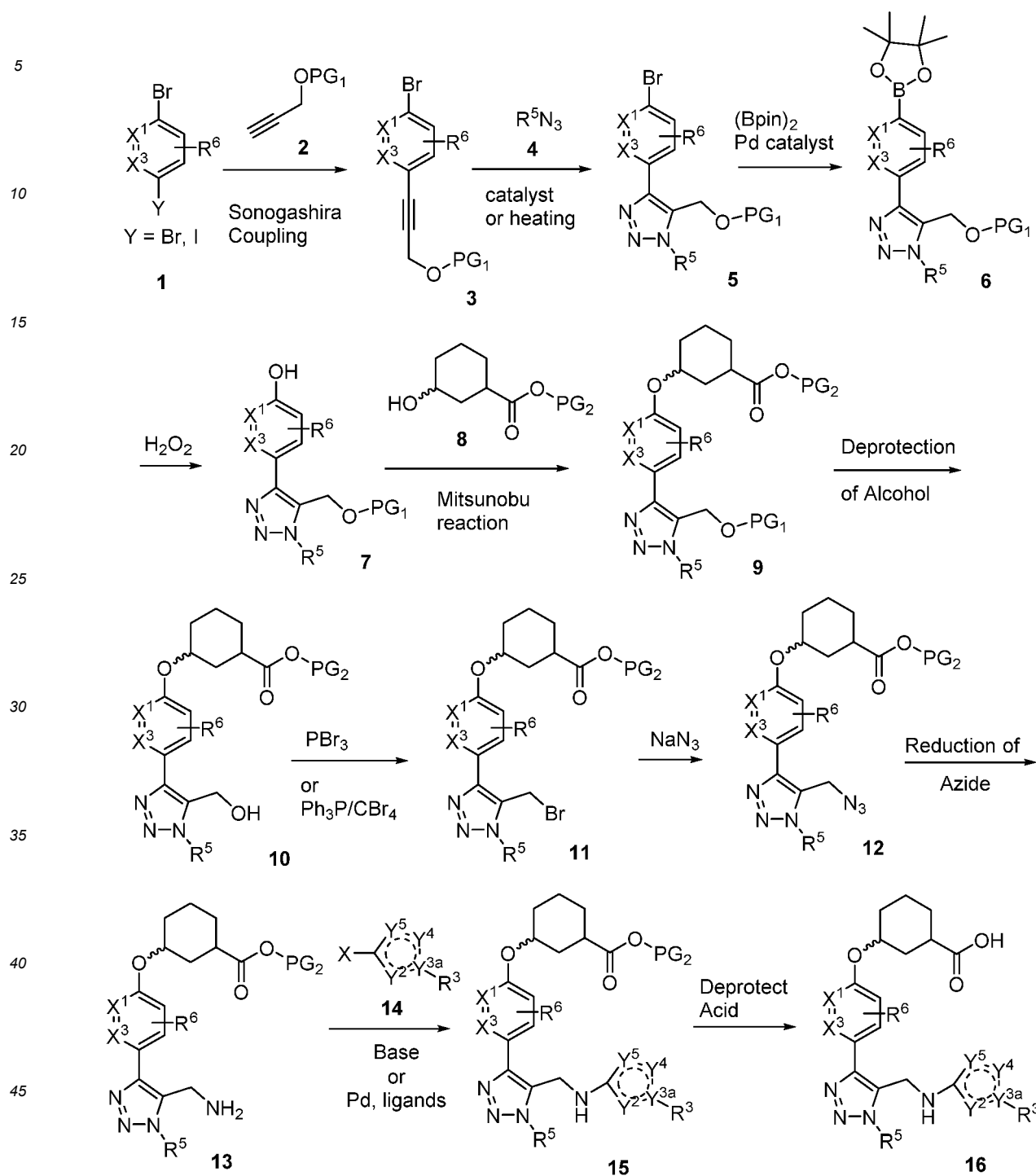
Scheme 1
