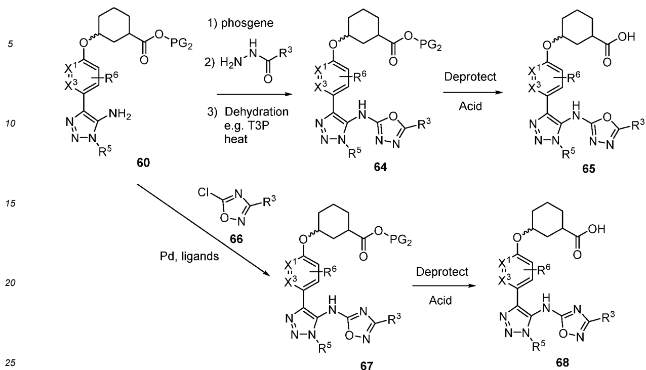
Scheme 13
