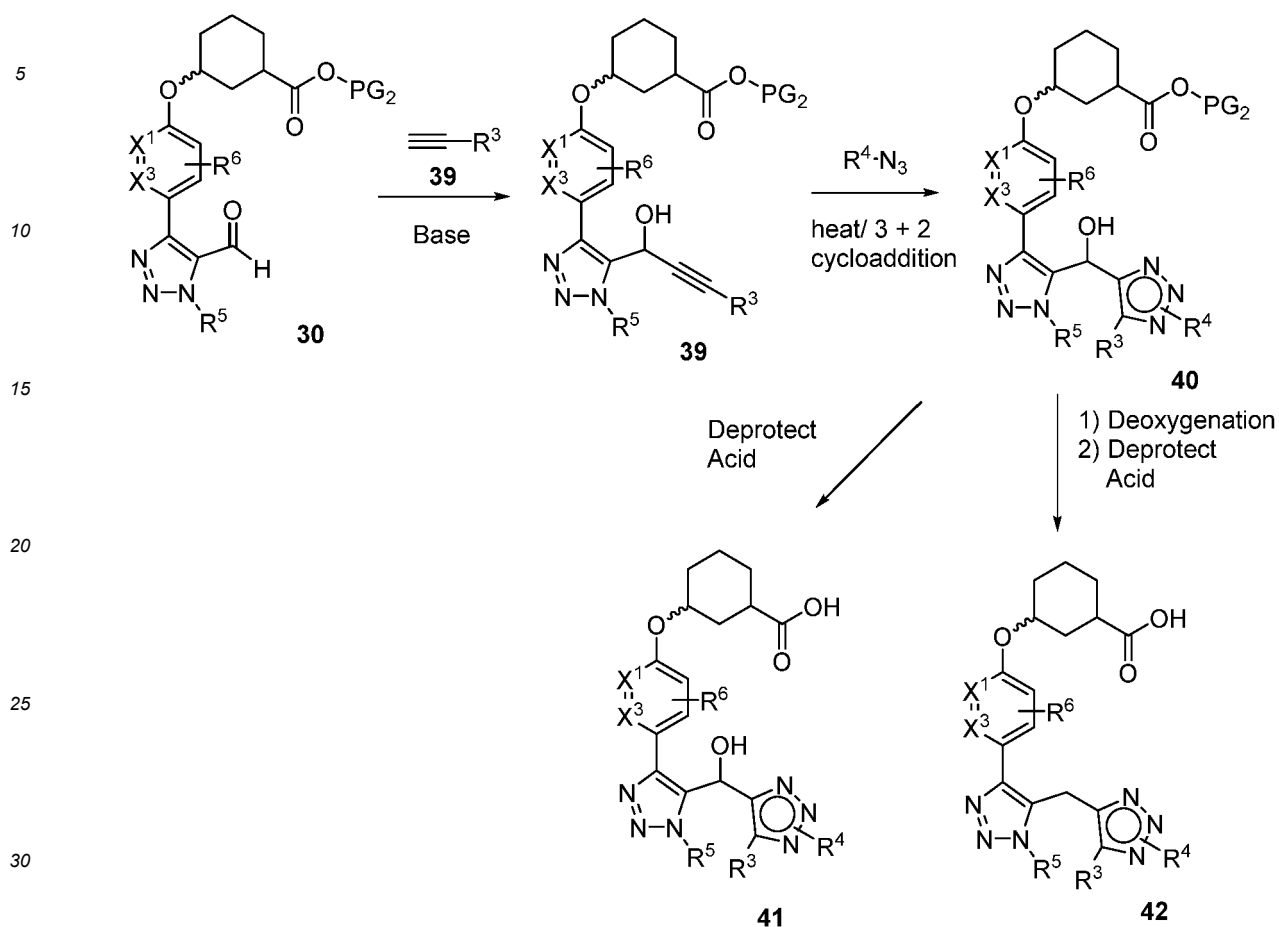
Scheme 7
