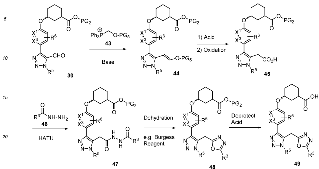
Scheme 8
