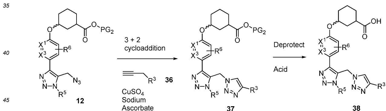
Scheme 6
