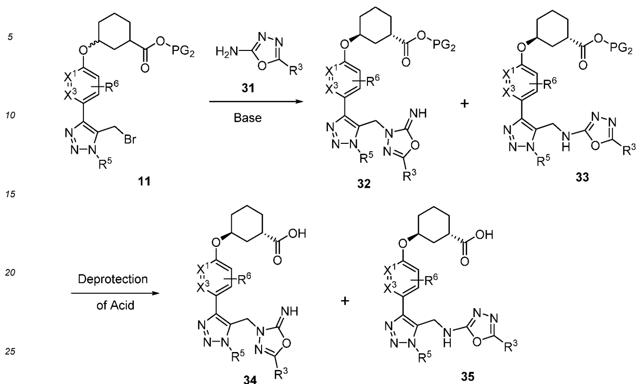
Scheme 5
