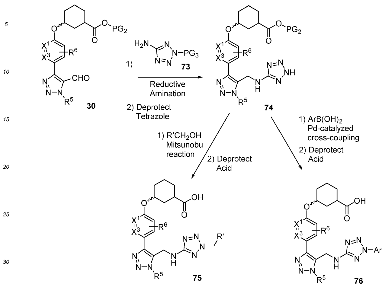
Scheme 15
