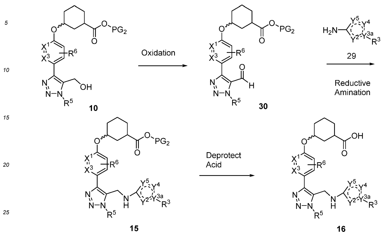
Scheme 4
