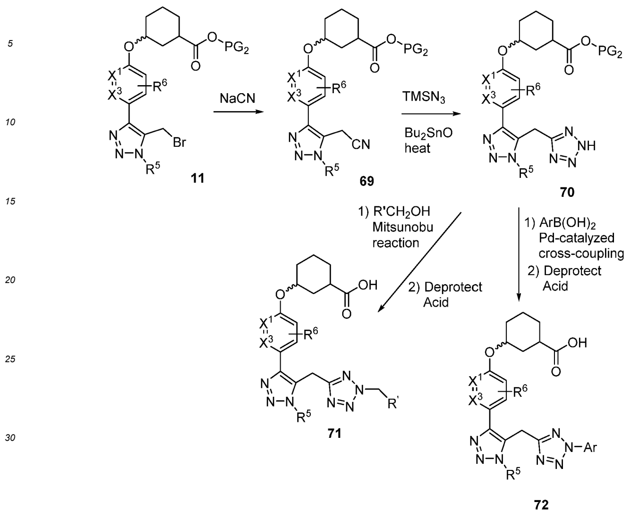
Scheme 14
