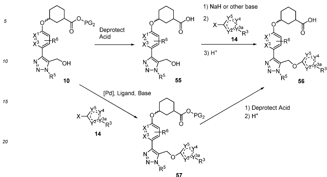
Scheme 10
