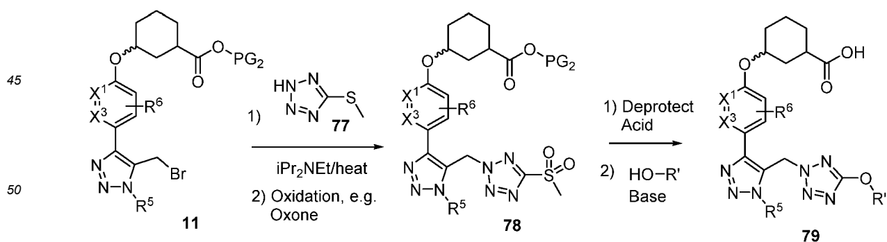
Scheme 16
