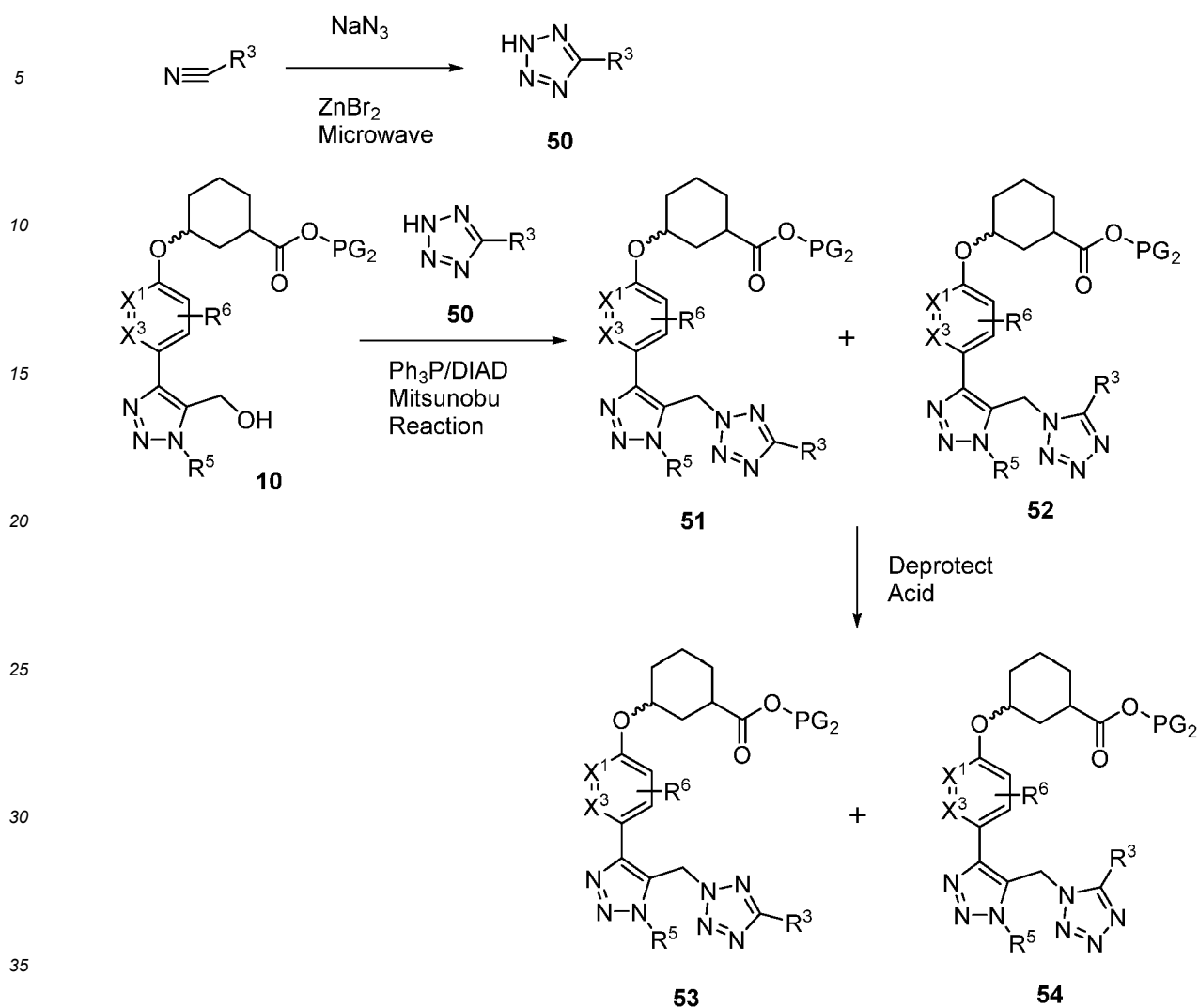
Scheme 9
