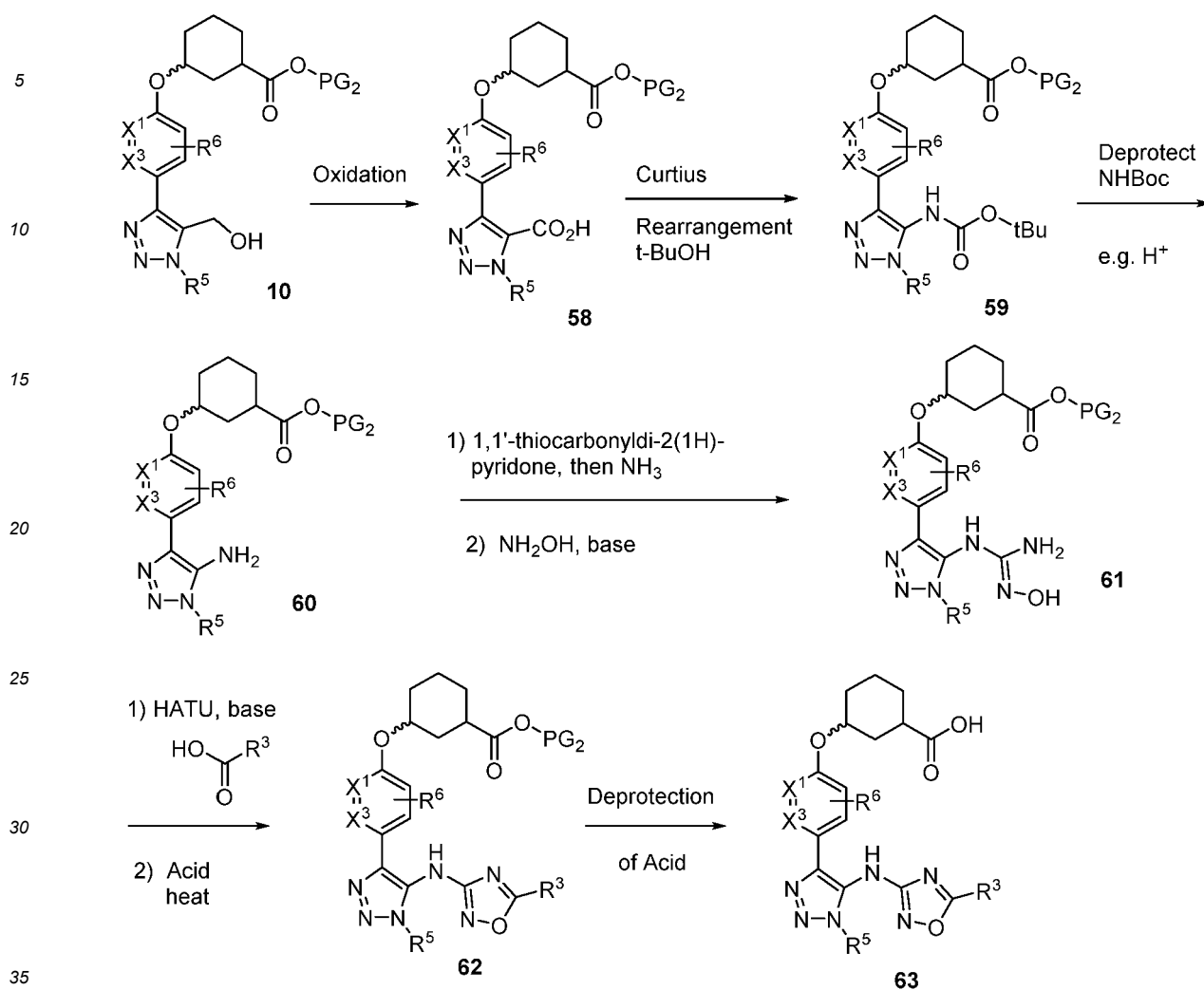
Scheme 12
