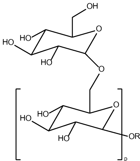
Alkyl Polyglucoside
