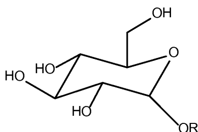
Alkyl Glucoside
