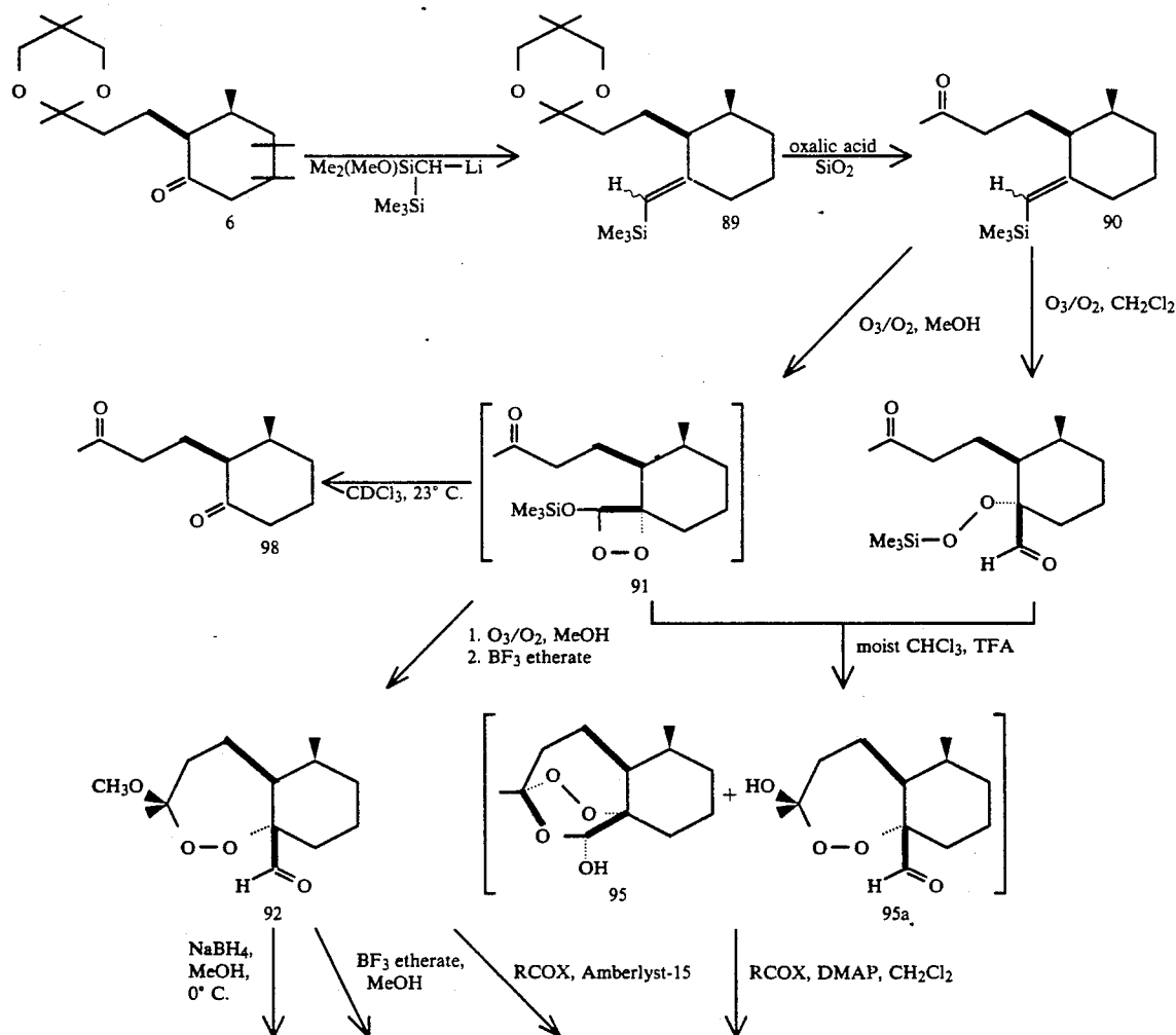
Scheme X
