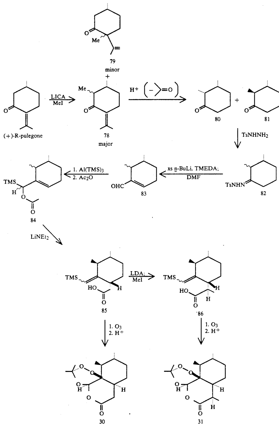
Scheme VIII
