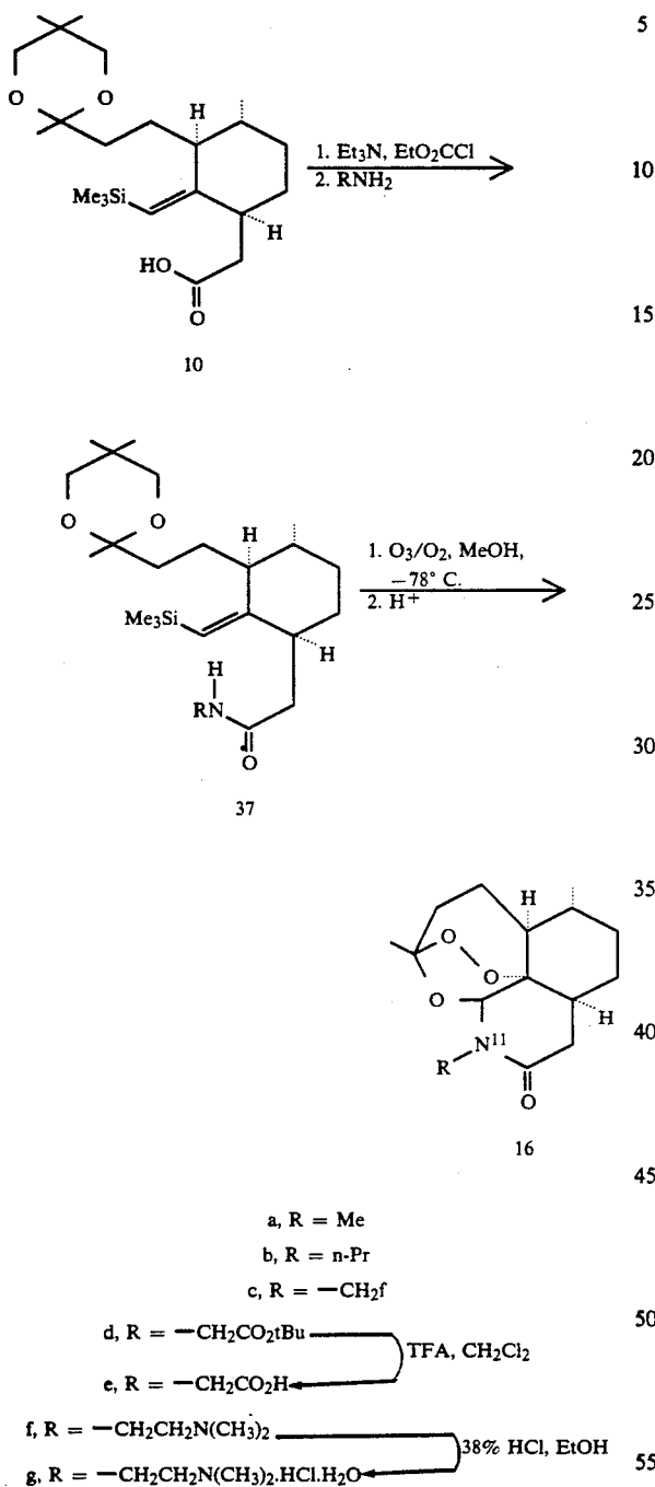
Scheme XI
