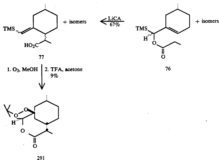
Scheme VII
