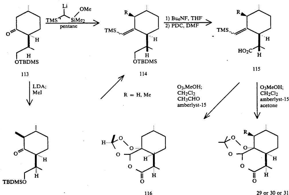
Scheme VIIa
