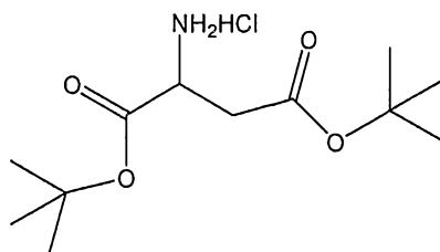
L-aspartic acid di-t-butyl ester hydrochloride
