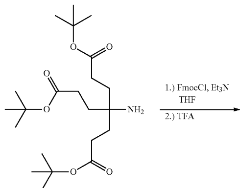
di-tert-butyl-4-amino-4-[2-(tert-butoxycarbonyl)ethyl]heptanedionate Chemical Formula: C_{22}H_{41}NO_6 Molecular Weight: 415.56
