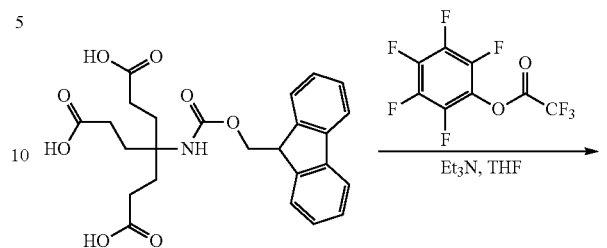
Chemical Formula: C_{25}H_{27}NO_8 Molecular Weight: 469.48
