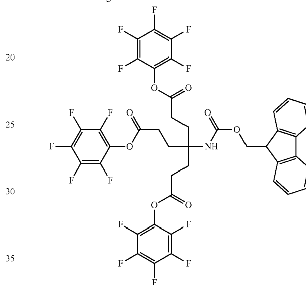
Chemical Formula: C_{43}H_{24}F_{15}NO_8 Molecular Weight: 967.63
