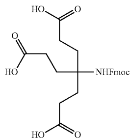
Chemical Formula: C_{37}H_{51}NO_8 Molecular Weight: 637.80
