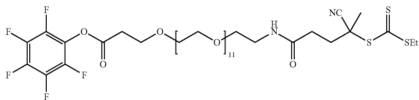
MD-03-30 Chemical Formula: \text{C}_{42}\text{H}_{63}\text{F}_5\text{N}_2\text{O}_{15}\text{S}_3 Molecular Weight: 1029.16
