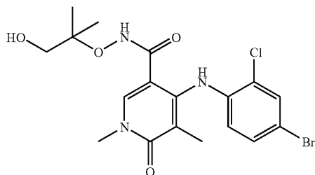
Example 68
