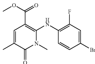
Methyl 2-(4-bromo-2-fluorophenylamino)-1,5-dimethyl-6-oxo-1,6-dihydropyridine-3-carboxylate
