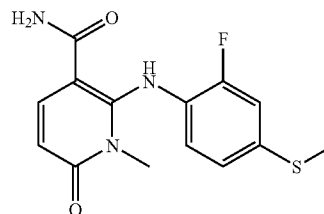
2-(2-fluoro-4-(methylthio)phenylamino)-1-methyl-6-oxo-1,6-dihydropyridine-3-carboxamide
