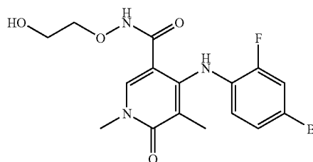
4-(4-Bromo-2-fluorophenylamino)-1,5-dimethyl-6-oxo-1,6-dihydropyridine-3-carboxylic acid (2-hydroxyethoxy)-amide
