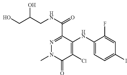
5-Chloro-N-(2,3-dihydroxypropyl)-4-(2-fluoro-4-iodophenylamino)-1-methyl-6-oxo-1,6-dihydropyridine-3-carboxamide
