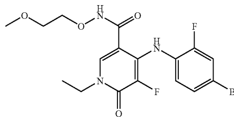
4-(4-Bromo-2-fluorophenylamino)-1-ethyl-5-fluoro-6-oxo-1,6-dihydropyridine-3-carboxylic acid (2-methoxyethoxy)-amide
