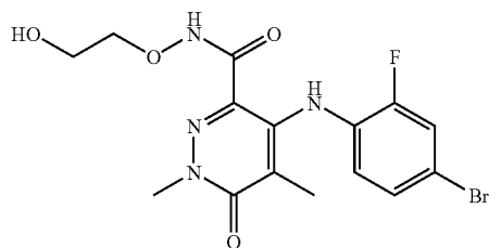
4-(4-Bromo-2-fluorophenylamino)-N-(2-hydroxyethoxy)-1,5-dimethyl-6-oxo-1,6-dihydropyridazine-3-carboxamide
