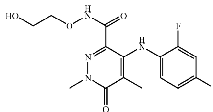
4-(2-Fluoro-4-iodophenylamino)-N-(2-hydroxyethoxy)-1,5-dimethyl-6-oxo-1,6-dihydropyridazine-3-carboxamide
