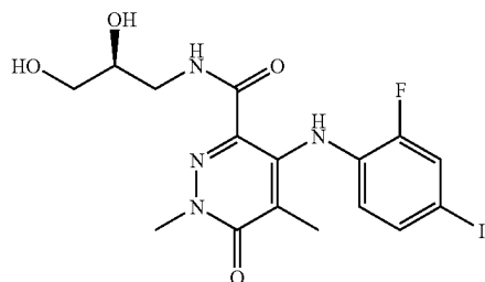
(S)-N-(2,3-Dihydroxypropyl)-4-(2-fluoro-4-iodophenylamino)-1,5-dimethyl-6-oxo-1,6-dihydropyridine-3-carboxamide
