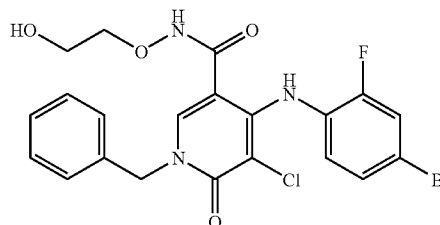
1-Benzyl-4-(4-bromo-2-fluorophenylamino)-5-chloro-6-oxo-1,6-dihydropyridine-3-carboxylic acid (2-hydroxyethoxy)-amide
