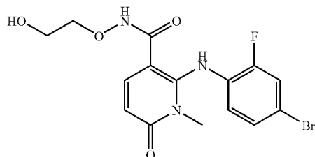
2-(4-Bromo-2-fluorophenylamino)-1-methyl-6-oxo-1,6-dihydropyridine-3-carboxylic acid (2-hydroxyethoxy)-amide
