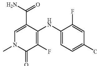
4-(4-Chloro-2-fluorophenylamino)-5-fluoro-1-methyl-6-oxo-1,6-dihydropyridine-3-carboxylic acid amide
