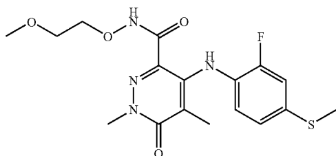
4-(2-Fluoro-4-(methylthio)phenylamino)-N-(2-methoxyethoxy)-1,5-dimethyl-6-oxo-1,6-dihydropyridazine-3-carboxamide
