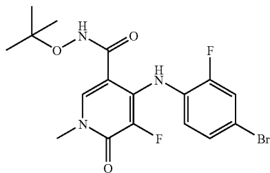
4-(4-Bromo-2-fluorophenylamino)-5-fluoro-1-methyl-6-oxo-1,6-dihydropyridine-3-carboxylic acid tert-butoxyamide
