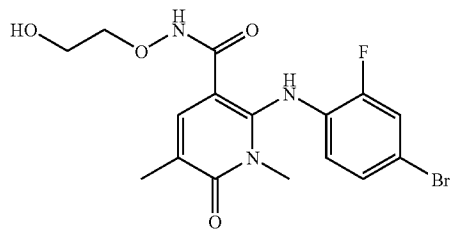
2-(4-Bromo-2-fluorophenylamino)-N-(2-hydroxyethoxy)-1,5-dimethyl-6-oxo-1,6-dihydropyridine-3-carboxamide
