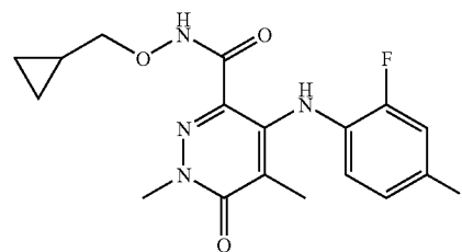
N-(Cyclopropylmethoxy)-4-(2-fluoro-4-iodophenylamino)-1,5-dimethyl-6-oxo-1,6-dihydropyridazine-3-carboxamide
