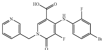
4-(4-Bromo-2-fluorophenylamino)-5-fluoro-6-oxo-1-pyridin-3-ylmethyl-1,6-dihydropyridine-3-carboxylic acid
