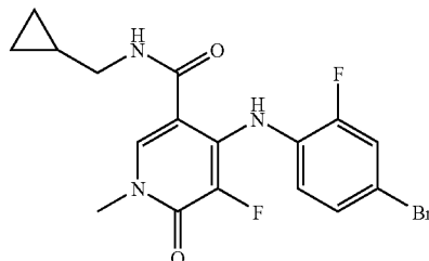
4-(4-Bromo-2-fluorophenylamino)-5-fluoro-1-methyl-6-oxo-1,6-dihydropyridine-3-carboxylic acid cyclopropylmethylamide
