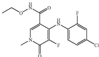
4-(4-Chloro-2-fluorophenylamino)-5-fluoro-1-methyl-6-oxo-1,6-dihydropyridine-3-carboxylic acid ethoxyamide
