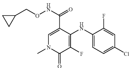
4-(4-Chloro-2-fluorophenylamino)-5-fluoro-1-methyl-6-oxo-1,6-dihydropyridine-3-carboxylic acid cyclopropylmethoxyamide
