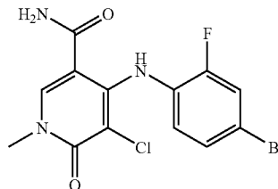
4-(4-Bromo-2-fluorophenylamino)-5-chloro-1-methyl-6-oxo-1,6-dihydropyridine-3-carboxylic acid amide
