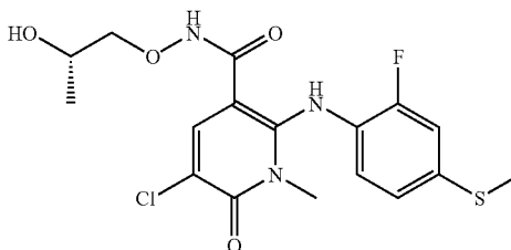
(S)-5-chloro-2-(2-fluoro-4-(methylthio)phenylamino)-N-(2-hydroxypropoxy)-1-methyl-6-oxo-1,6-dihydropyridine-3-carboxamide
