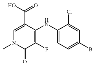
4-(4-Bromo-2-chlorophenylamino)-5-fluoro-1-methyl-6-oxo-1,6-dihydropyridine-3-carboxylic acid
