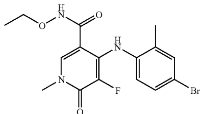
4-(4-Bromo-2-methylphenylamino)-5-fluoro-1-methyl-6-oxo-1,6-dihydropyridine-3-carboxylic acid ethoxyamide
