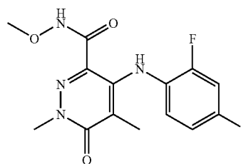
4-(2-Fluoro-4-iodophenylamino)-N-methoxy-1,5-dimethyl-6-oxo-1,6-dihydropyridazine-3-carboxamide
