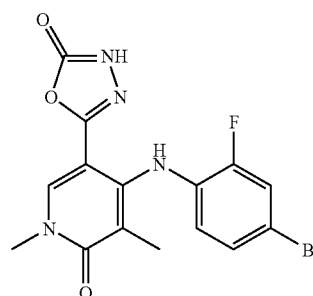
4-(4-Bromo-2-fluorophenylamino)-1,3-dimethyl-5-(5-oxo-4,5-dihydro-[1,3,4]oxadiazol-2-yl)-1H-pyridin-2-one
