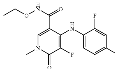
5-Fluoro-4-(2-fluoro-4-methylphenylamino)-1-methyl-6-oxo-1,6-dihydropyridine-3-carboxylic acid ethoxyamide
