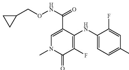
5-Fluoro-4-(2-fluoro-4-methylphenylamino)-1-methyl-6-oxo-1,6-dihydropyridine-3-carboxylic acid cyclopropylmethoxyamide
