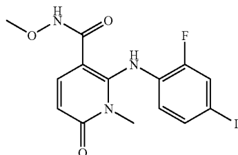
2-(2-Fluoro-4-iodophenylamino)-1-methyl-6-oxo-1,6-dihydropyridine-3-carboxylic acid methoxyamide
