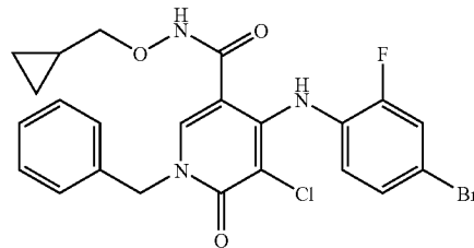
1-Benzyl-4-(4-bromo-2-fluorophenylamino)-5-chloro-6-oxo-1,6-dihydropyridine-3-carboxylic acid cyclopropylmethoxyamide
