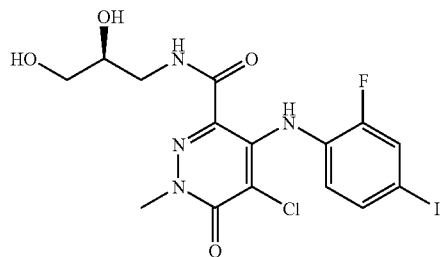
(S)-5-Chloro-N-(2,3-dihydroxypropyl)-4-(2-fluoro-4-iodophenylamino)-1-methyl-6-oxo-1,6-dihydropyridine-3-carboxamide
