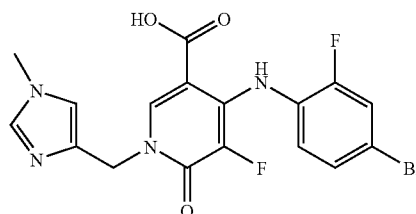
4-(4-Bromo-2-fluorophenylamino)-5-fluoro-1-(1-methyl-1H-imidazol-4-ylmethyl)-6-oxo-1,6-dihydropyridine-3-carboxylic acid
