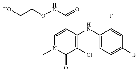
4-(4-Bromo-2-fluorophenylamino)-5-chloro-1-methyl-6-oxo-1,6-dihydropyridine-3-carboxylic acid (2-hydroxyethoxy)-amide
