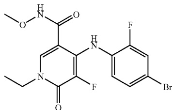
Example 56
