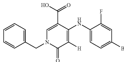
1-Benzyl-4-(4-bromo-2-fluorophenylamino)-6-oxo-1,6-dihydropyridine-3-carboxylic acid
