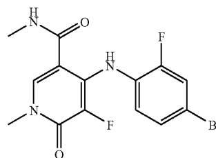
4-(4-Bromo-2-fluorophenylamino)-5-fluoro-1-methyl-6-oxo-1,6-dihydropyridine-3-carboxylic acid methylamide
