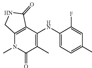
4-(2-Fluoro-4-methylphenylamino)-1,3-dimethyl-6,7-dihydro-1H-pyrrolo[3,4-b]pyridine-2,5-dione
