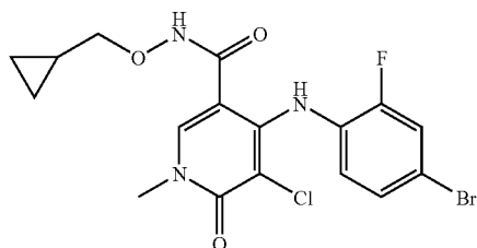
4-(4-Bromo-2-fluorophenylamino)-5-chloro-1-methyl-6-oxo-1,6-dihydropyridine-3-carboxylic acid cyclopropylmethoxy amide
