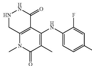
4-(2-Fluoro-4-methylphenylamino)-1,3-dimethyl-7,8-dihydro-1H,6H-pyrido[2,3-d]pyridazine-2,5-dione
