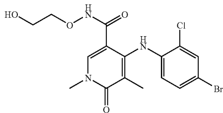
Example 69
