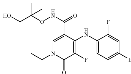
4-(4-Bromo-2-fluorophenylamino)-1-ethyl-5-fluoro-6-oxo-1,6-dihydropyridine-3-carboxylic acid (2-hydroxy-1,1-dimethylethoxy)-amide
