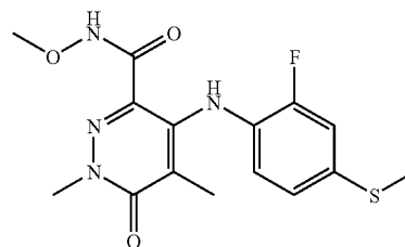
4-(2-Fluoro-4-(methylthio)phenylamino)-N-methoxy-1,5-dimethyl-6-oxo-1,6-dihydropyridazine-3-carboxamide
