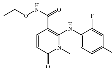
N-ethoxy-2-(2-fluoro-4-iodophenylamino)-1-methyl-6-oxo-1,6-dihydropyridine-3-carboxamide
