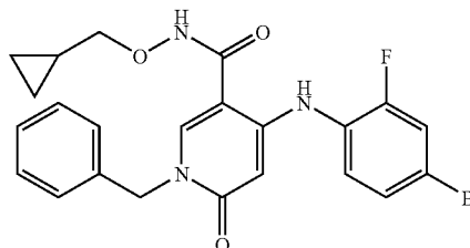
1-Benzyl-4-(4-bromo-2-fluorophenylamino)-6-oxo-1,6-dihydropyridine-3-carboxylic acid cyclopropylmethoxy amide
