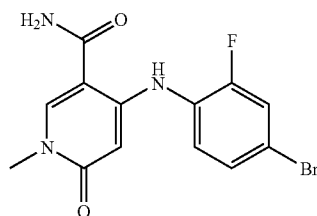
4-(4-Bromo-2-fluorophenylamino)-1-methyl-6-oxo-1,6-dihydropyridine-3-carboxylic acid amide
