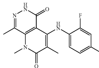
4-(2-Fluoro-4-methylphenylamino)-1,3,8-trimethyl-1H,6H-pyrido[2,3-d]pyridazine-2,5-dione
