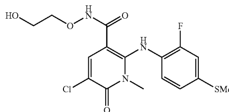
5-chloro-2-(2-fluoro-4-(methylthio)phenylamino)-N-(2-hydroxyethoxy)-1-methyl-6-oxo-1,6-dihydropyridine-3-carboxamide
