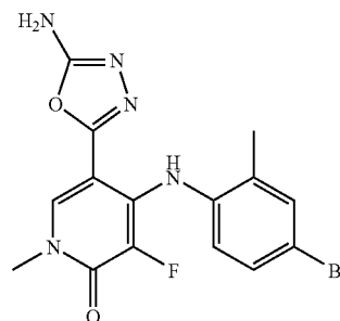
5-(5-Amino-[1,3,4]oxadiazol-2-yl)-4-(4-bromo-2-methylphenylamino)-3-fluoro-1-methyl-1H-pyridin-2-one
