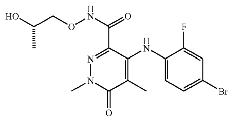
(S)-4-(4-Bromo-2-fluorophenylamino)-N-(2-hydroxypropoxy)-1,5-dimethyl-6-oxo-1,6-dihydropyridazine-3-carboxamide
