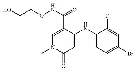
4-(4-Bromo-2-fluorophenylamino)-1-methyl-6-oxo-1,6-dihydropyridine-3-carboxylic acid (2-hydroxyethoxy)-amide
