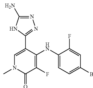
5-(5-Amino-4H-[1,2,4]triazol-3-yl)-4-(4-bromo-2-fluorophenylamino)-3-fluoro-1-methyl-1H-pyridin-2-one
