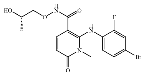
(S)-2-(4-bromo-2-fluorophenylamino)-N-(2-hydroxypropoxy)-1-methyl-6-oxo-1,6-dihydropyridine-3-carboxamide
