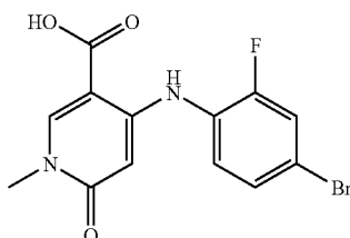
4-(4-Bromo-2-fluorophenylamino)-1-methyl-6-oxo-1,6-dihydropyridine-3-carboxylic acid
