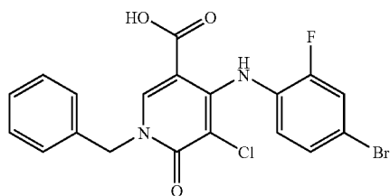
1-Benzyl-4-(4-bromo-2-fluorophenylamino)-5-chloro-6-oxo-1,6-dihydropyridine-3-carboxylic acid
