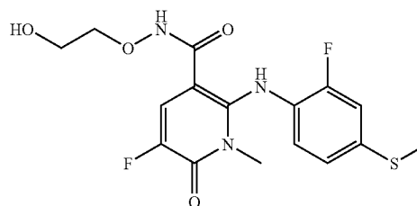
5-fluoro-2-(2-fluoro-4-(methylthio)phenylamino)-N-(2-hydroxyethoxy)-1-methyl-6-oxo-1,6-dihydropyridine-3-carboxamide
