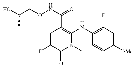
(S)-5-fluoro-2-(2-fluoro-4-(methylthio)phenylamino)-N-(2-hydroxypropoxy)-1-methyl-6-oxo-1,6-dihydropyridine-3-carboxamide
