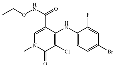
4-(4-Bromo-2-fluorophenylamino)-5-chloro-1-methyl-6-oxo-1,6-dihydropyridine-3-carboxylic acid ethoxyamide
