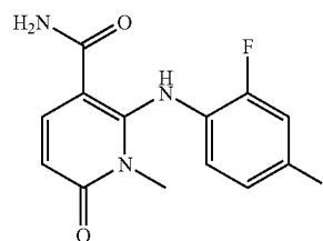
2-(2-fluoro-4-iodophenylamino)-1-methyl-6-oxo-1,6-dihydropyridine-3-carboxamide
