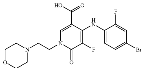
4-(4-Bromo-2-fluorophenylamino)-5-fluoro-1-(2-morpholin-4-yl-ethyl)-6-oxo-1,6-dihydropyridine-3-carboxylic acid
