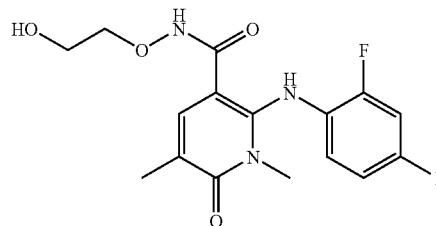
2-(2-fluoro-4-iodophenylamino)-N-(2-hydroxyethoxy)-1,5-dimethyl-6-oxo-1,6-dihydropyridine-3-carboxamide
