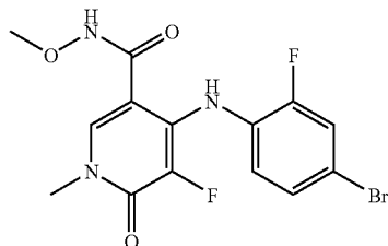
4-(4-Bromo-2-fluorophenylamino)-5-fluoro-1-methyl-6-oxo-1,6-dihydropyridine-3-carboxylic acid methoxyamide
