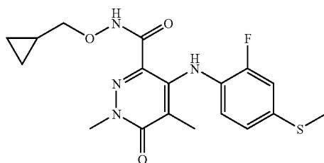
N-(Cyclopropylmethoxy)-4-(2-fluoro-4-(methylthio)phenylamino)-1,5-dimethyl-6-oxo-1,6-dihydropyridazine-3-carboxamide
