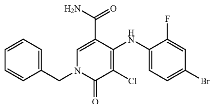
1-Benzyl-4-(4-bromo-2-fluorophenylamino)-5-chloro-6-oxo-1,6-dihydropyridine-3-carboxylic acid amide
