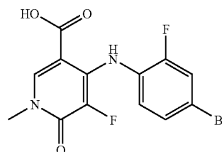
4-(4-Bromo-2-fluorophenylamino)-5-fluoro-1-methyl-6-oxo-1,6-dihydropyridine-3-carboxylic acid
