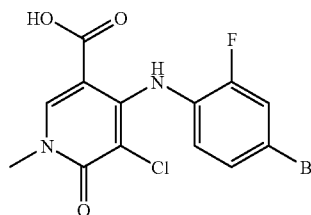
4-(4-Bromo-2-fluorophenylamino)-5-chloro-1-methyl-6-oxo-1,6-dihydropyridine-3-carboxylic acid
