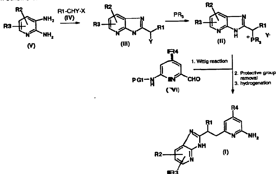
Reaction scheme 1:
