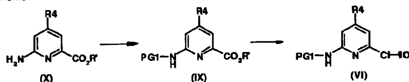
Reaction scheme 3:
