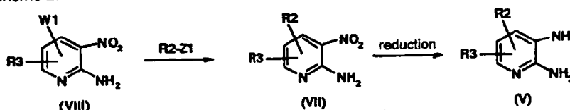
Reaction scheme 2:
