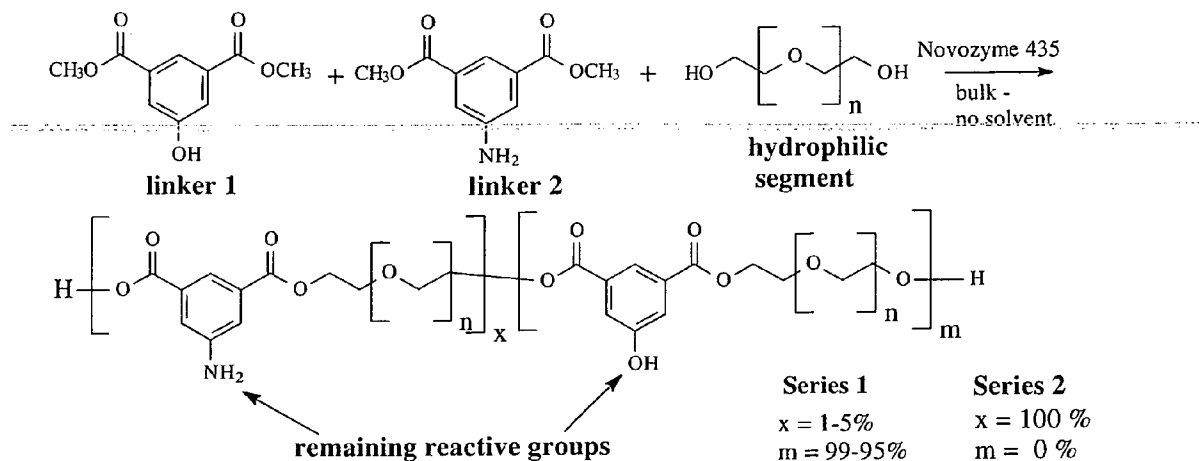
Figure 9. First stage of synthesis: enzymatic polymerization
