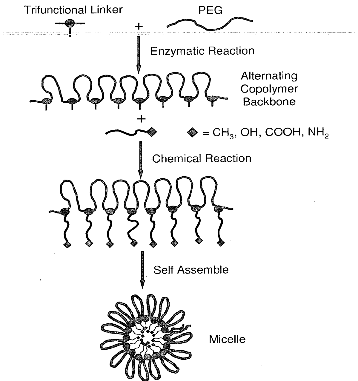
Figure 2. Formation of self-assembling alternating copolymer micelles
