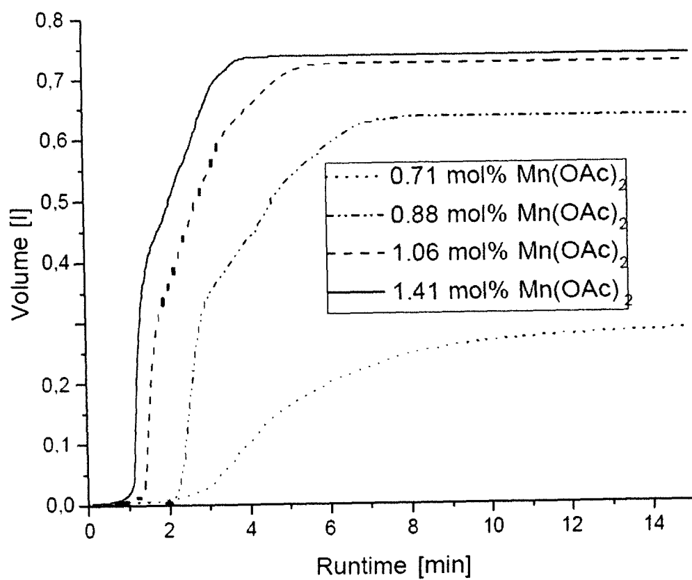
Fig. 12: Oxygen evolution from 5 g UHP using different concentrations of \text{Mn}(\text{OAc})_2 in BMIMOAac.
