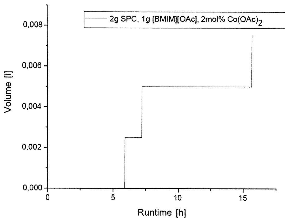
Fig. 16: Oxygen liberation from SPC in BMIMOAc.
