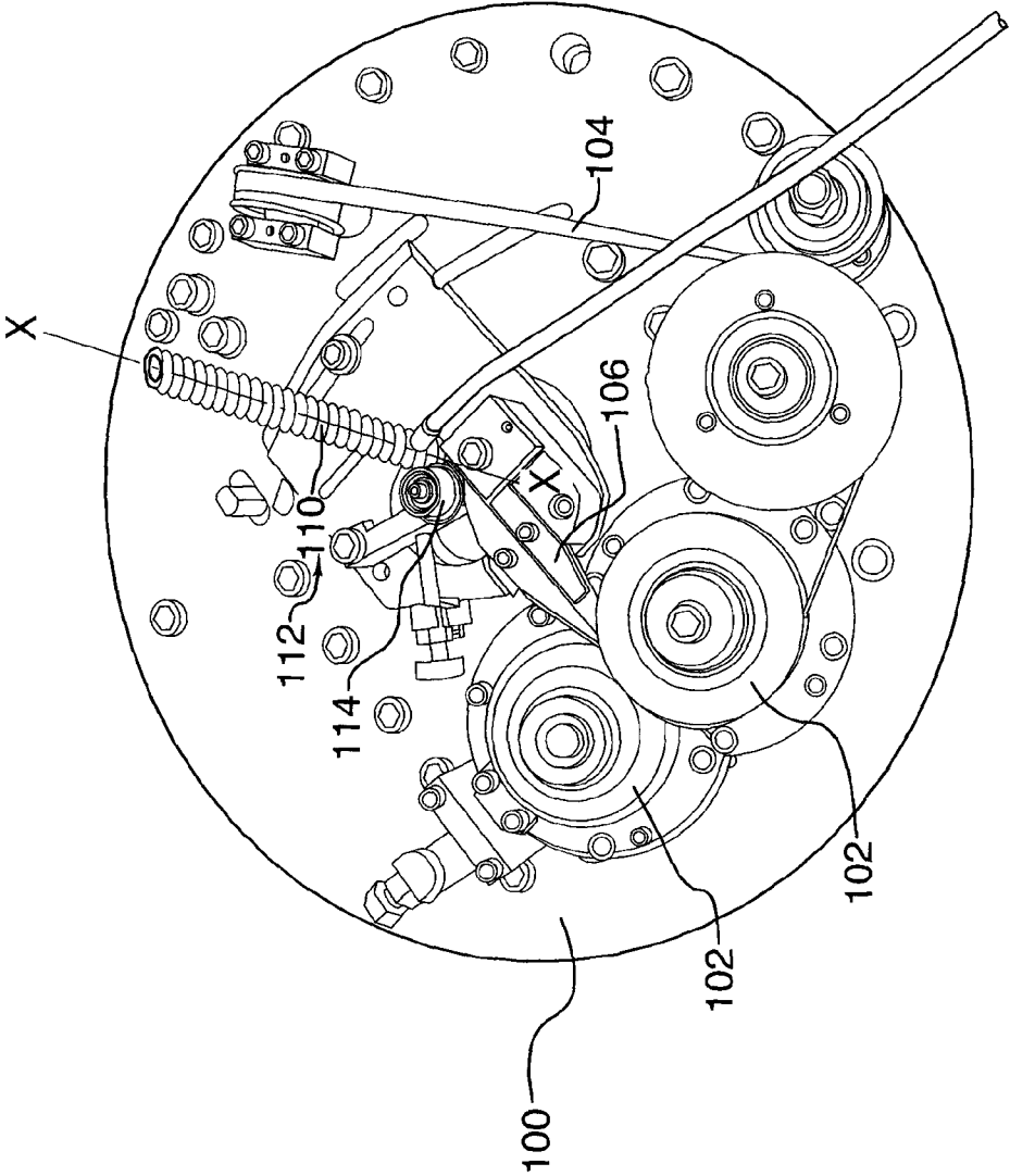
FIG. 1 (PRIOR ART)
