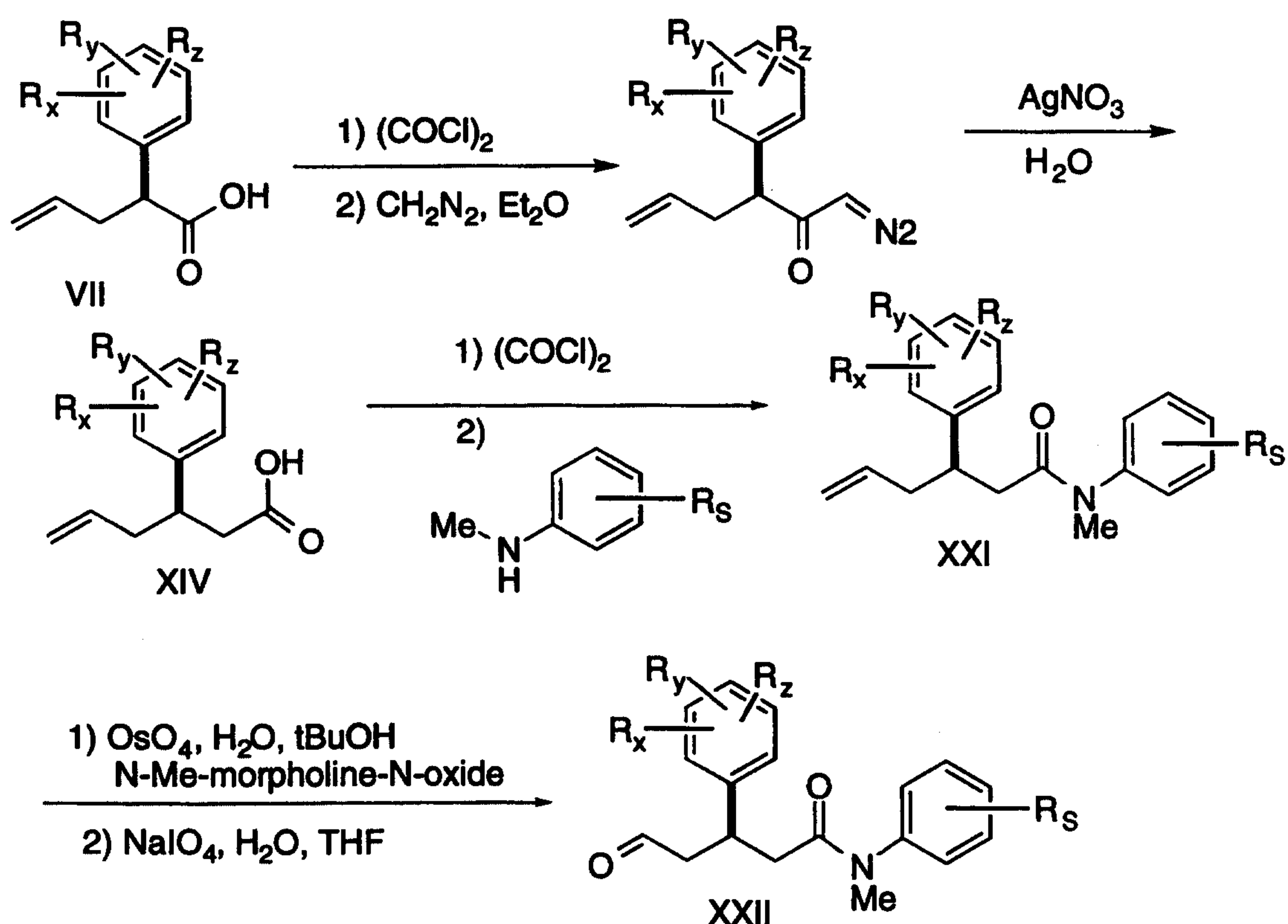
SCHEME 5
