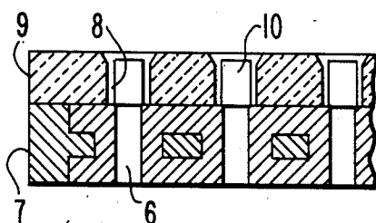
FIG. 3 PRIOR ART
