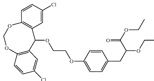
3-(4-[2-(2,10-Dichloro-12H-5,7-dioxo-dibenzo[a,d]cycloocten-12-yloxy)-ethoxy]-phenyl)-2-ethoxy-propionic acid ethyl ester
