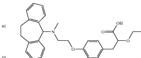
3-(4-[2-([10,11-dihydro-5H-dibenzo[a,d]cyclohepten-5-yl]-methyl-amino)-ethoxy]-phenyl)-2-ethoxypropanoic acid
