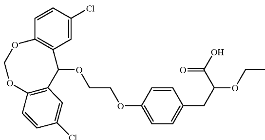
3-(4-[2-(2,10-Dichloro-12H-5,7-dioxo-dibenzo[a,d]cycloocten-12-yloxy)-ethoxy]-phenyl)-2-ethoxy-propionic acid
