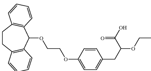
3-(4-[2-(10,11-Dihydro-5H-dibenzo[a,d]cyclohepten-5-yloxy)-ethoxy]-phenyl)-2-ethoxypropanoic acid
