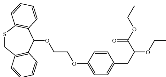
3-(4-[2-(6,11-Dihydrodibenzo[b,e]thiepin-11-yloxy)-ethoxy]-phenyl)-2-ethoxy-propionic acid ethyl ester a)
