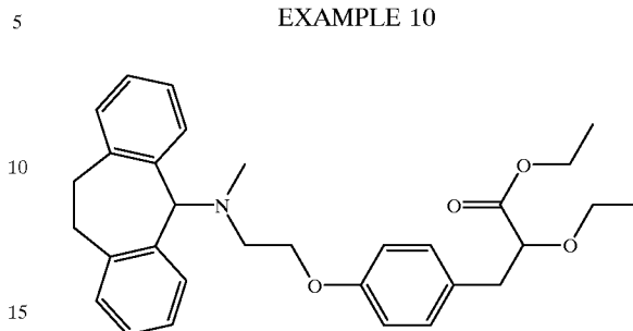
3-(4-[2-([10,11-dihydro-5H-dibenzo[a,d]cyclohepten-5-yl]-methyl-amino)-ethoxy]-phenyl)-2-ethoxypropanoic acid ethyl ester
