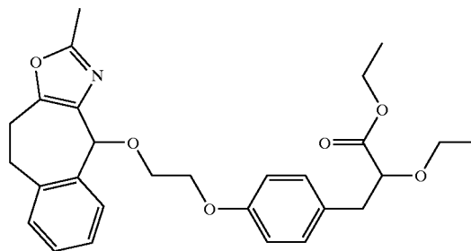
2-Ethoxy-3-(4-[2-(2-methyl-9,10-dihydro-4H-1-oxa-3-aza-benzo[f]azulen-4-yloxy)-ethoxy]-phenyl)-propionic acid ethyl ester
