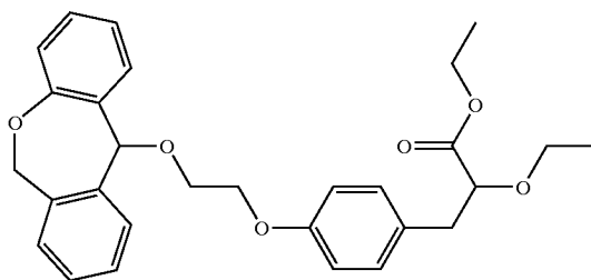
3-(4-[2-(6,11-Dihydrodibenzo[b,e]oxepin-11-yloxy)-ethoxy]-phenyl)-2-ethoxy-propionic acid ethyl ester
