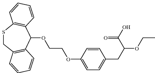
3-(4-[2-(6,11-Dihydrodibenzo[b,e]thiepin-11-yloxy)-ethoxy]-phenyl)-2-ethoxy-propionic acid
