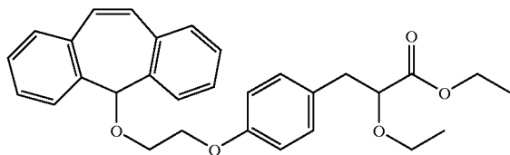
3-(4-[2-[5H-Dibenzo[a,d]cyclohepten-5-yloxy]-ethoxy]-phenyl)-2-ethoxy-propionic acid ethyl ester a)
