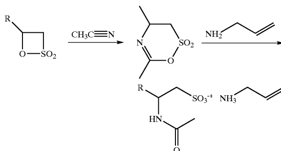
Scheme VII: 2-Acetamidoalkyl-1-Sulfonic Acid Allyl Amine Salts
