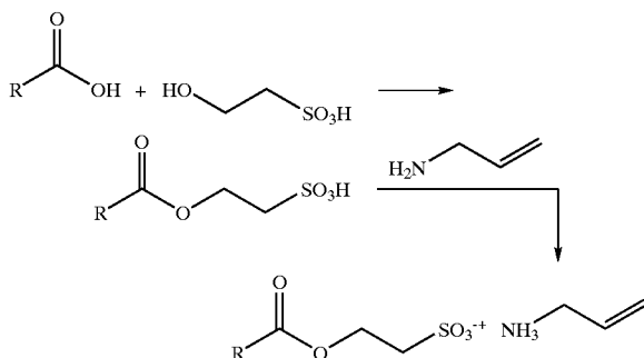
Scheme VI: Formation Of A Isethionic Acid Ethylenically Unsaturated Amine Salt
