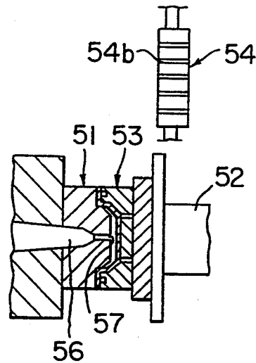
PRIOR ART FIG. 22
