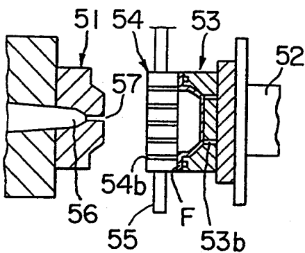
PRIOR ART FIG. 20
