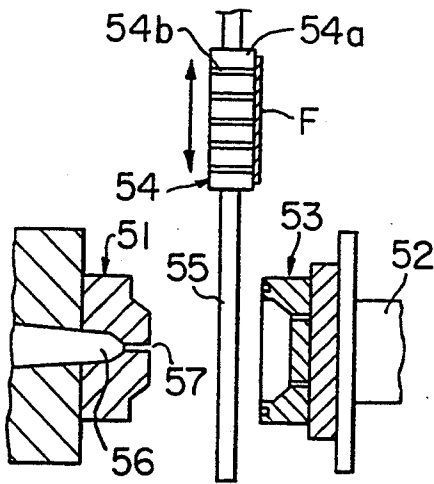
PRIOR ART FIG. 18
