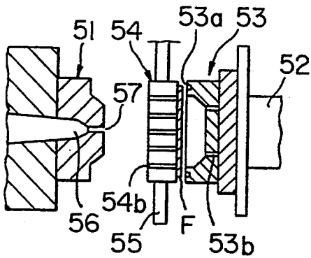
PRIOR ART FIG. 19
