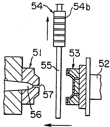
PRIOR ART FIG. 21
