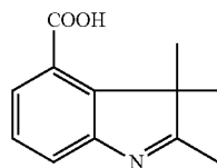
1.2 2,3,3-Trimethyl-4-carboxy-3H-indole
