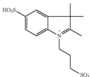
1.10 1-(3-Sulfonatopropyl)-2,3,3-trimethylindoleninium-5-sulfonate
