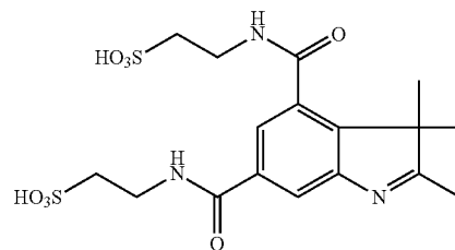
2,3,3-Trimethyl-4,6-di(sulfoethylcarboxyamido)-3H-indole
