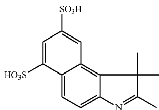
1,1,2-Trimethylbenz[e]indole-6,8-disulfonate
