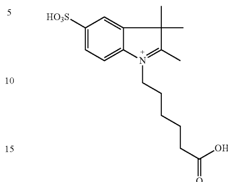
1.11 1-Carboxypentyl-2,3,3-trimethylindoleninium-5-sulfonate
