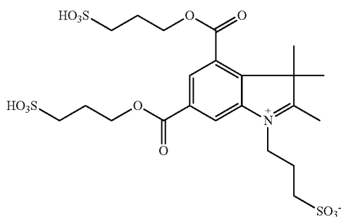
1-(3-Sulfonatopropyl)-2,3,3-trimethylindoleninium- 4,6-di(sulfonatopropylcarboxylate)
