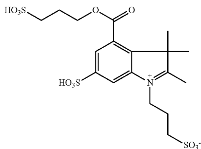
1-(3-Sulfonatopropyl)-2,3,3-trimethylindoleninium- 4-(sulfonatopropylcarboxylate)-6-sulfonate
