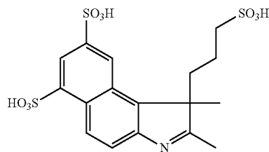
1,2-Dimethyl-1-(3-sulfopropyl)benz[e]indole-6,8-disulfonate
