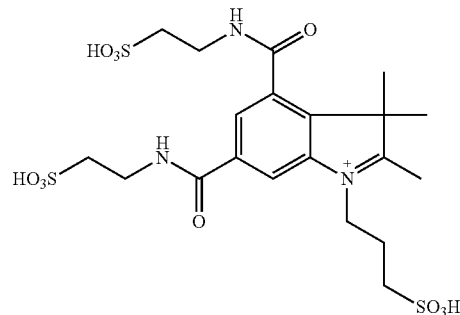
1-(3-Sulfopropyl)-2,3,3-trimethylindoleninium-4,6-di(sulfoethylcarboxyamido)
