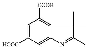
2,3,3-Trimethyl-4,6-dicarboxy-3H-indole
