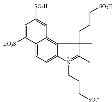
1,2-Dimethyl-1,3-bis(3-sulfopropyl)benz[e]indole-6,8-disulfonate
