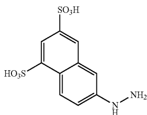
6-Hydrazino-1,3-naphthalenedisulfonate
