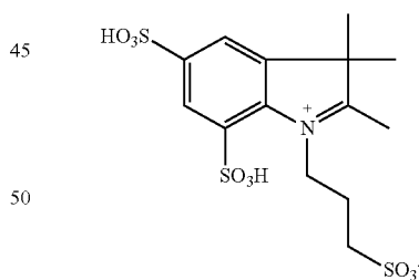
1.10 1-(3-Sulfonatopropyl)-2,3,3-trimethylindoleninium-5-sulfonate
