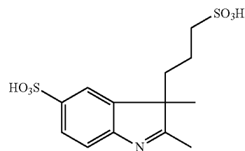
2,3-Dimethyl-3-(3-sulfopropyl)indoleninium-5-sulfonate
