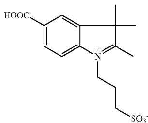
1.9 1-(3-Sulfonatopropyl)-2,3,3-trimethylindoleninium-5-carboxylate
