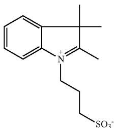
1-(3-Sulfonatopropyl)-2,3,3-trimethylindoleninium
