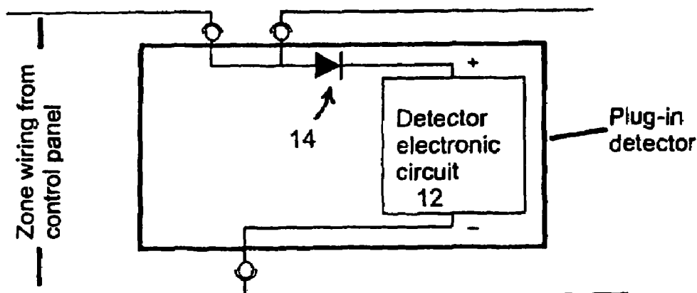
Fig 3 Polarity protection using series diode
