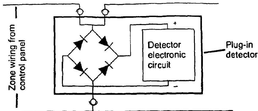
Polarity protection using diode bridge
