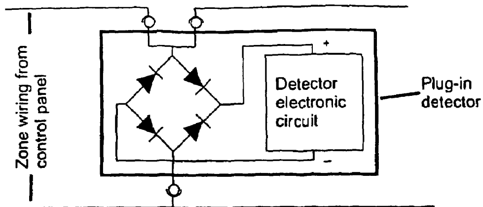
Fig 1 Polarity protection using diode bridge
