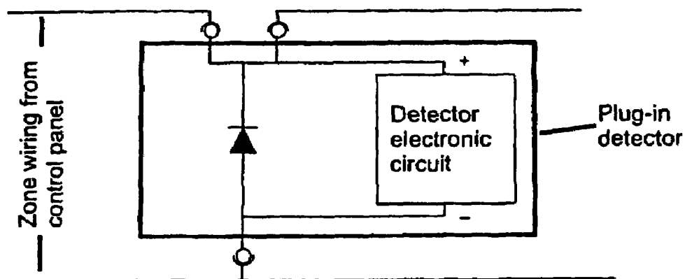
Fig 2 Polarity protection using shunt diode
