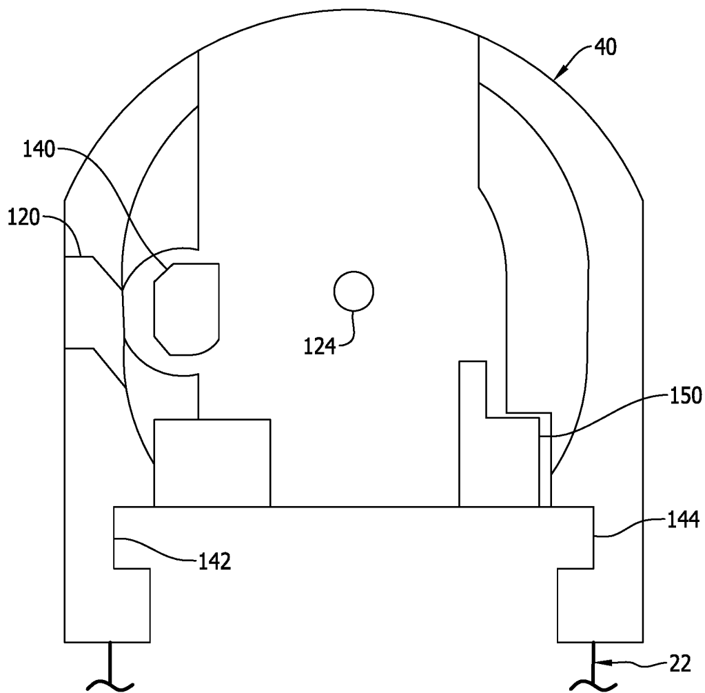
FIG. 3 (PRIOR ART)
