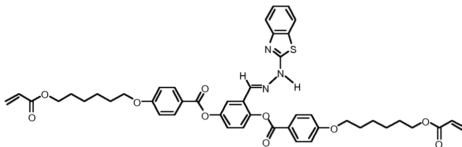
Compound A
