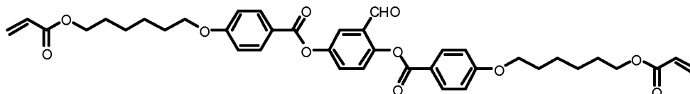
Intermediate D
