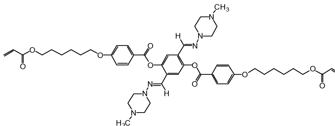
Compound 2
