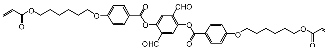
Intermediate C
