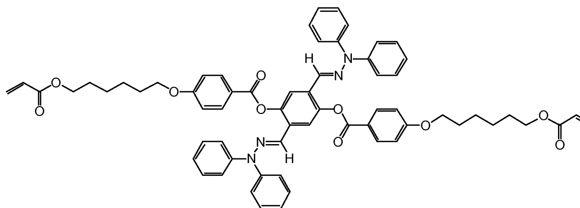
Compound 3
