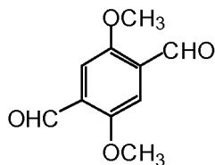
Intermediate A
