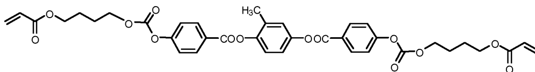
Compound 2r
