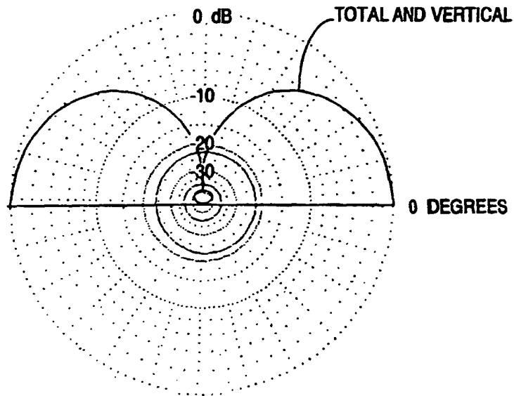
FIGURE 7D-3B (PRIOR ART)
