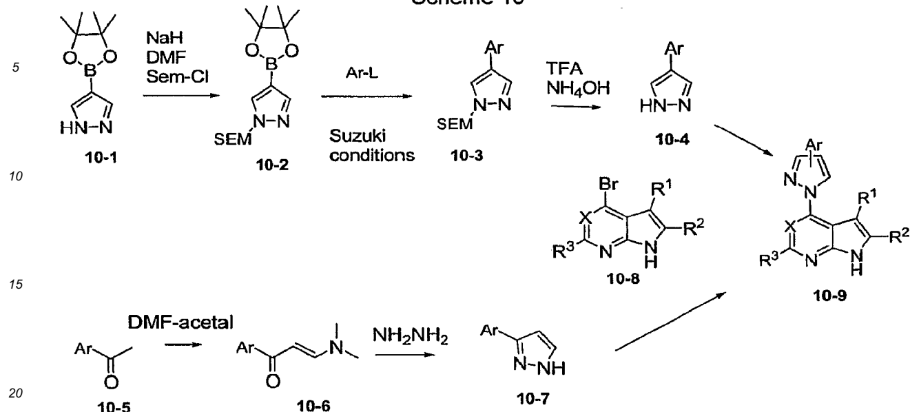
Scheme 10
