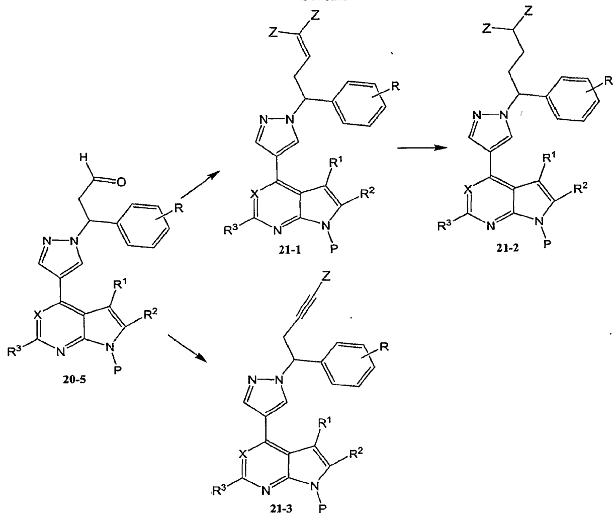
Scheme 21
