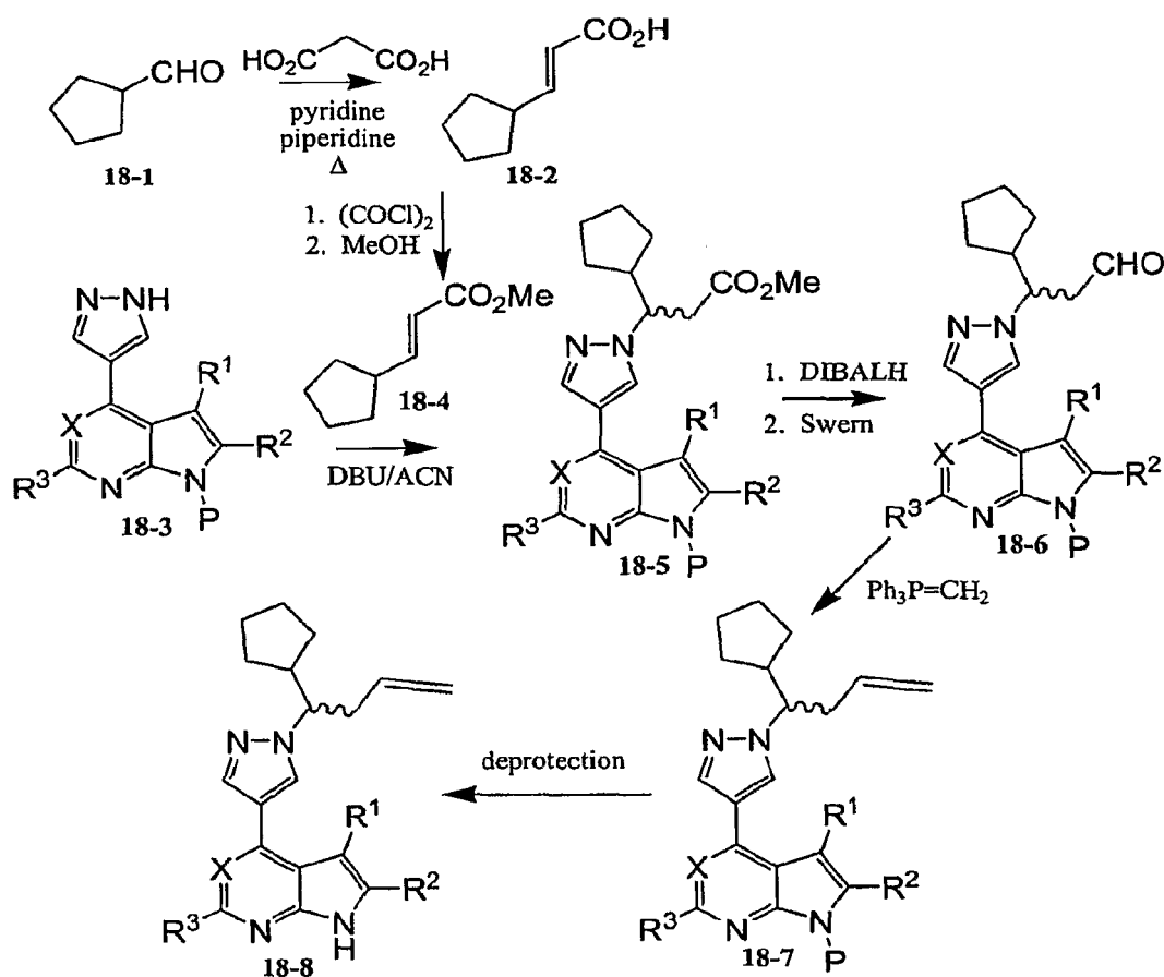
Scheme 18
