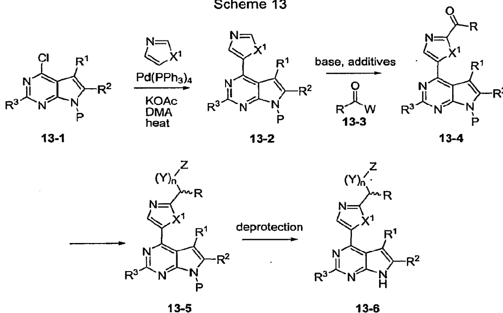
Scheme 13
