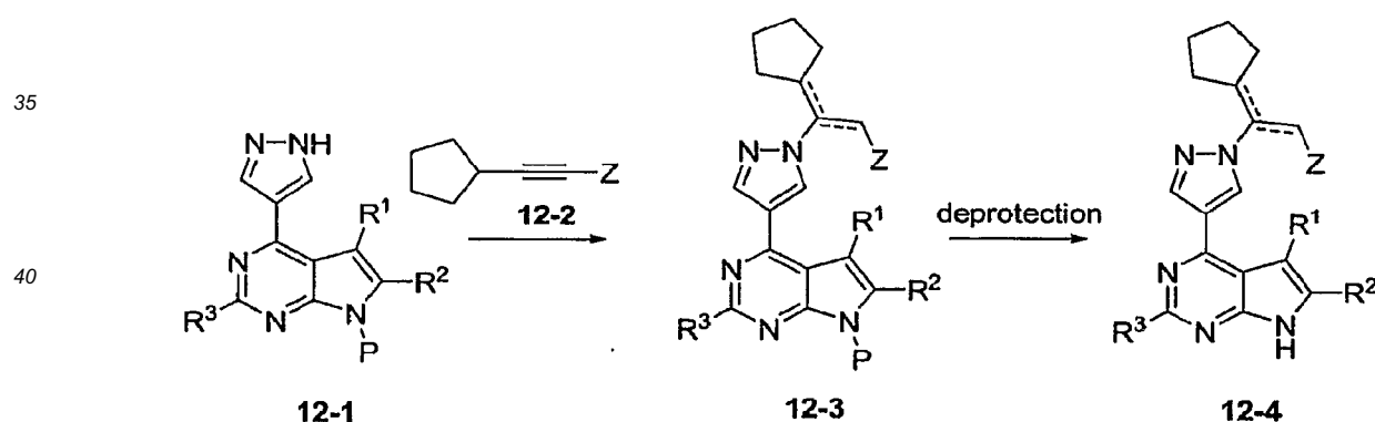
Scheme 12
