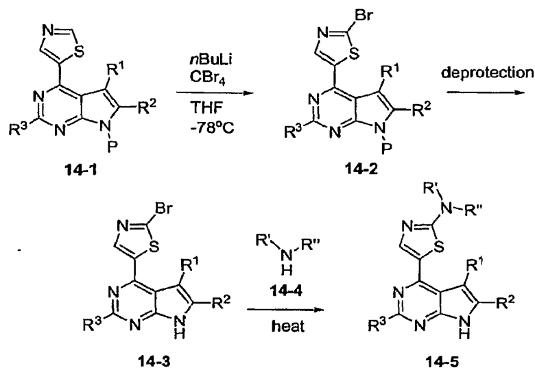
Scheme 14
