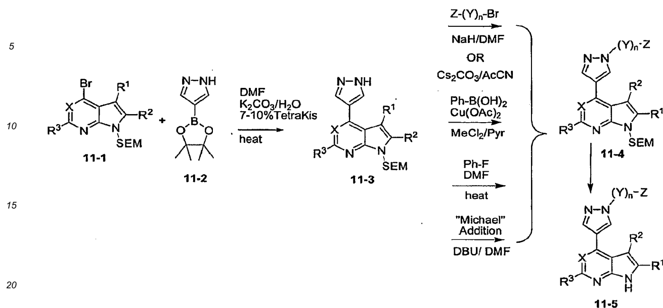
Scheme 11
