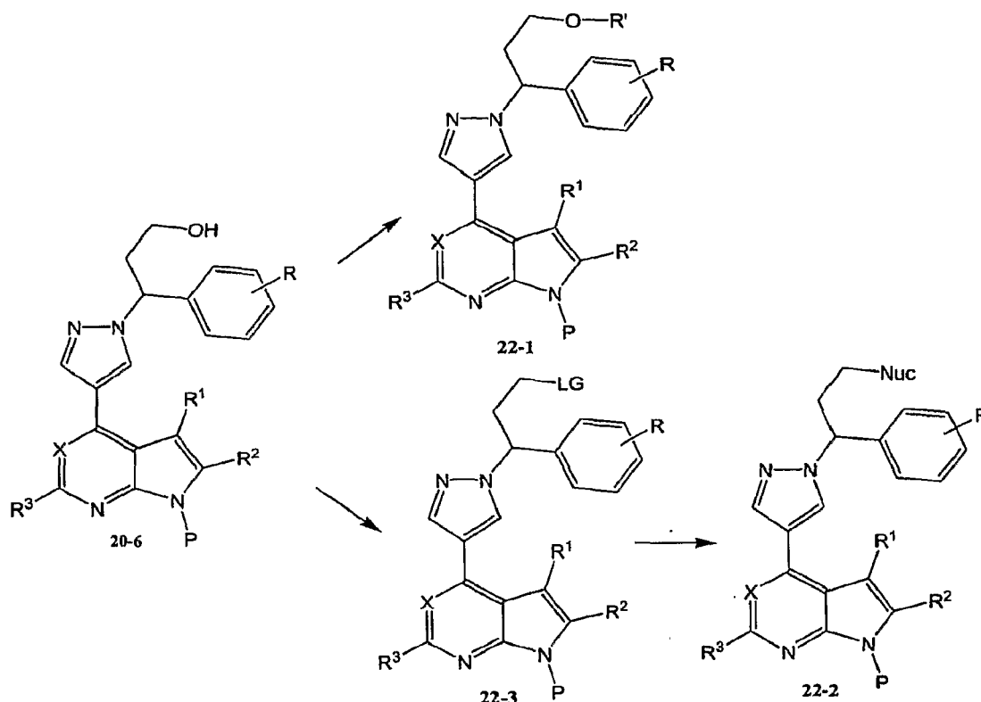
Scheme 22
