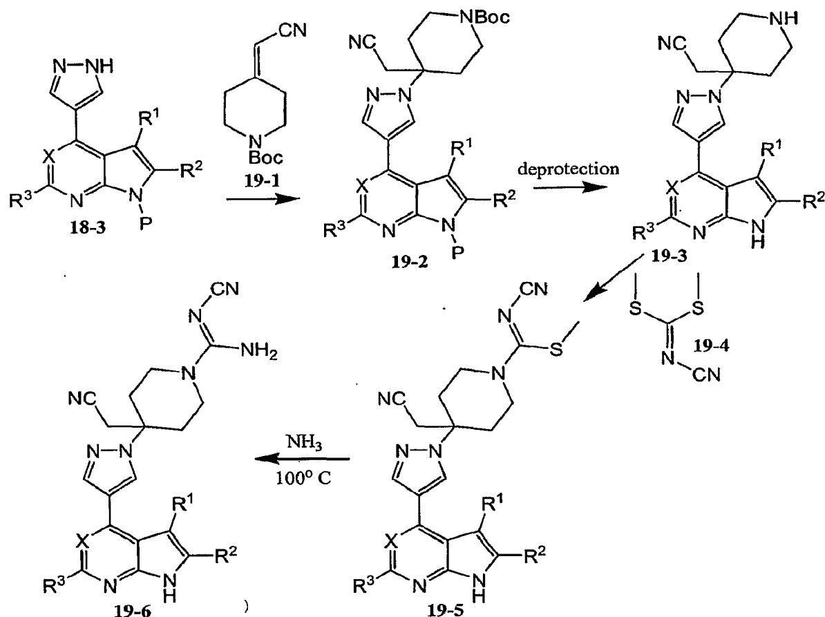
Scheme 19
