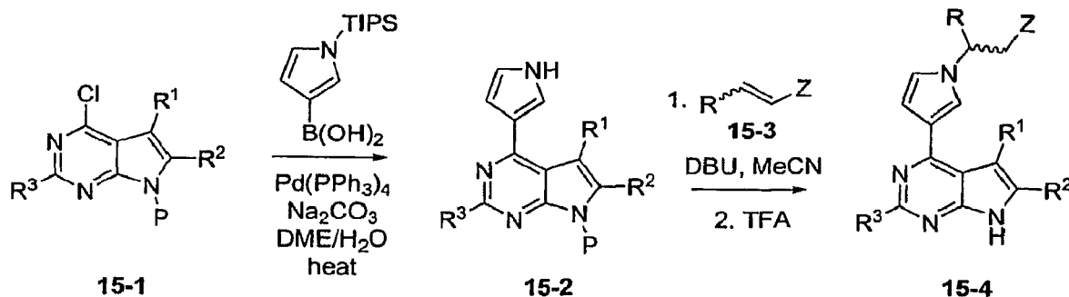
Scheme 15
