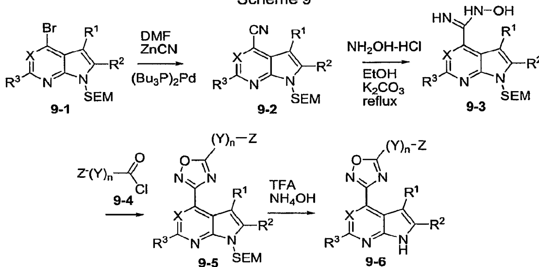
Scheme 9
