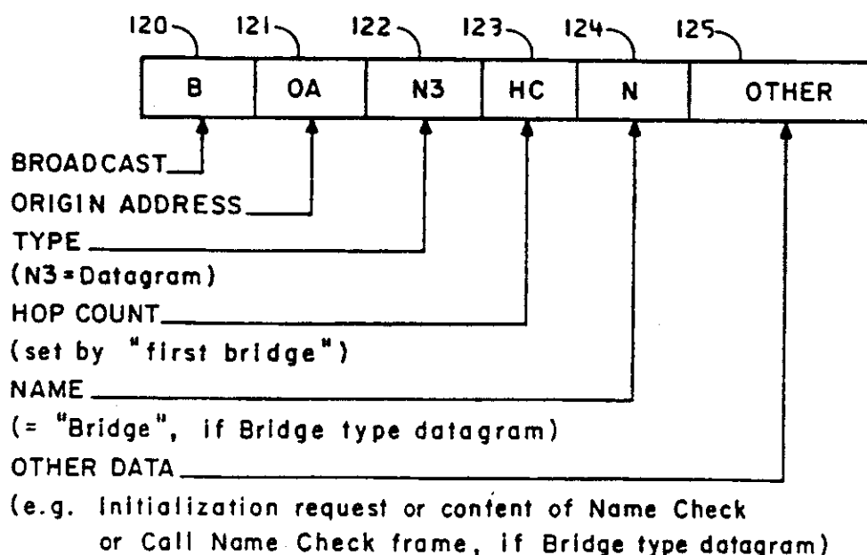
FIG. 4 (BRIDGE DATAGRAM)
