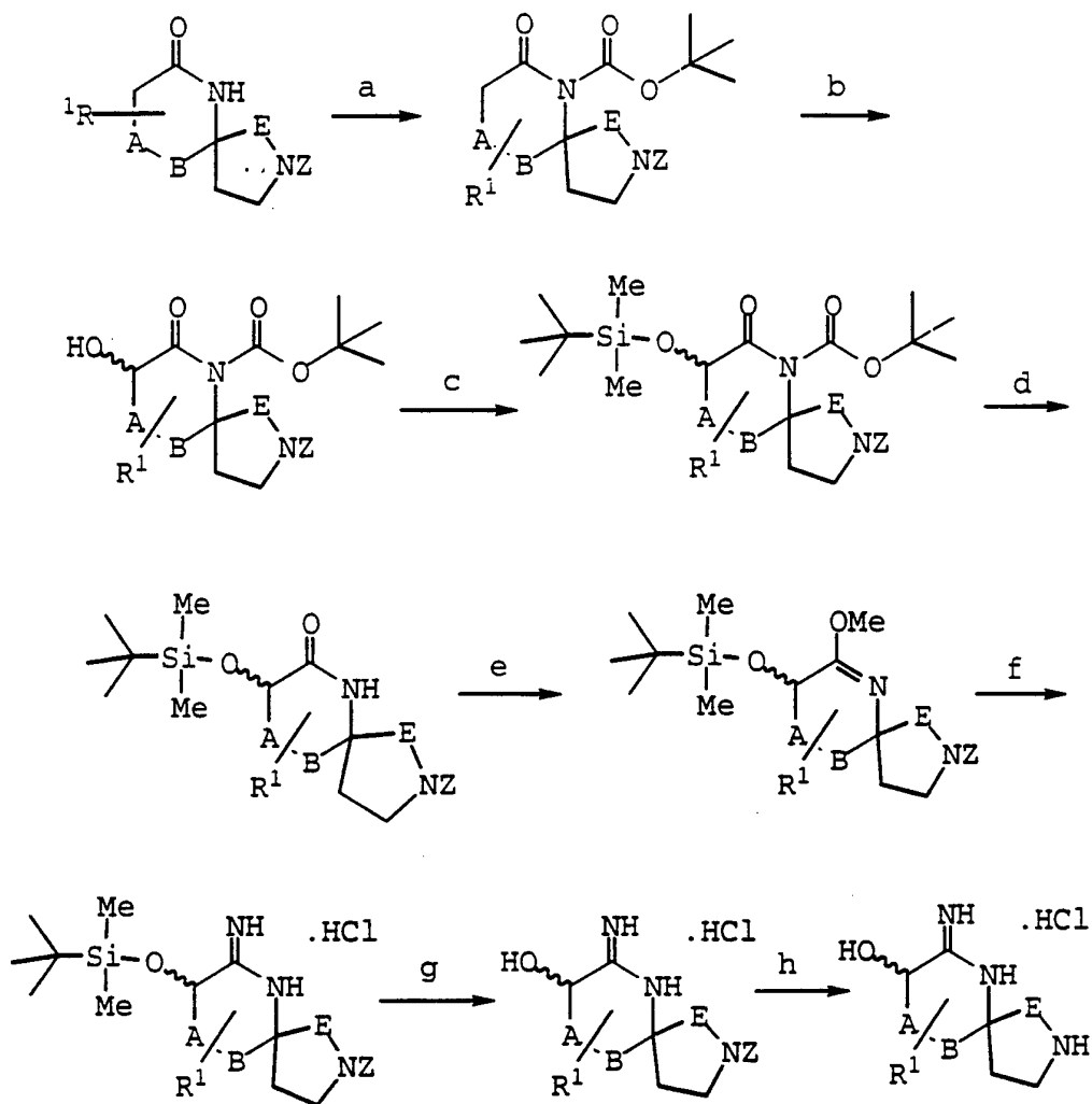
Scheme 10:
