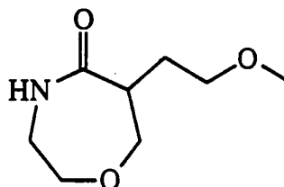
Isomer B
