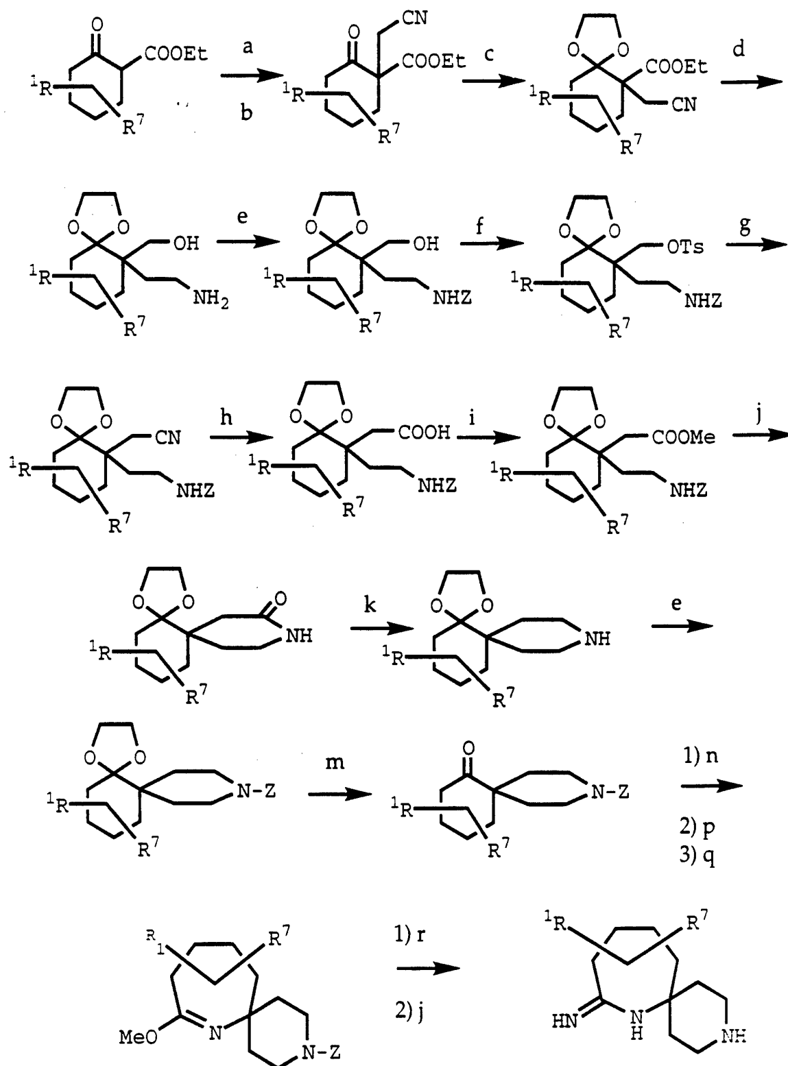
Scheme 7:
