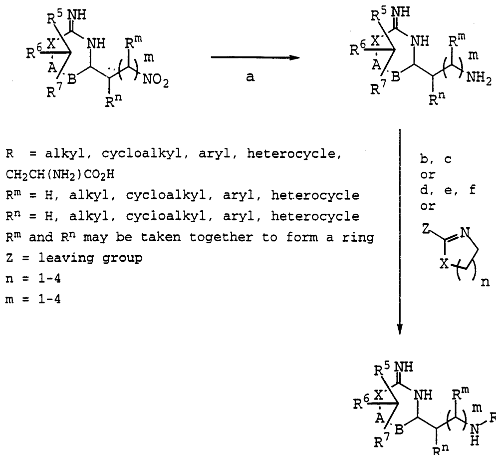
Scheme 11:
