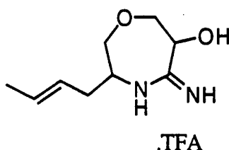
Isomer A
