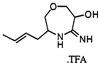
Isomer B
