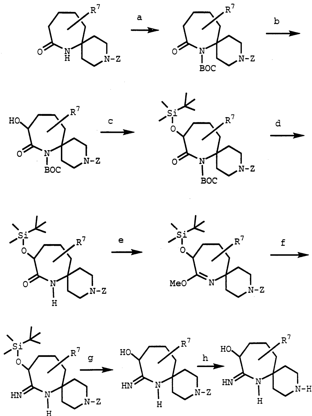
Scheme 8:
