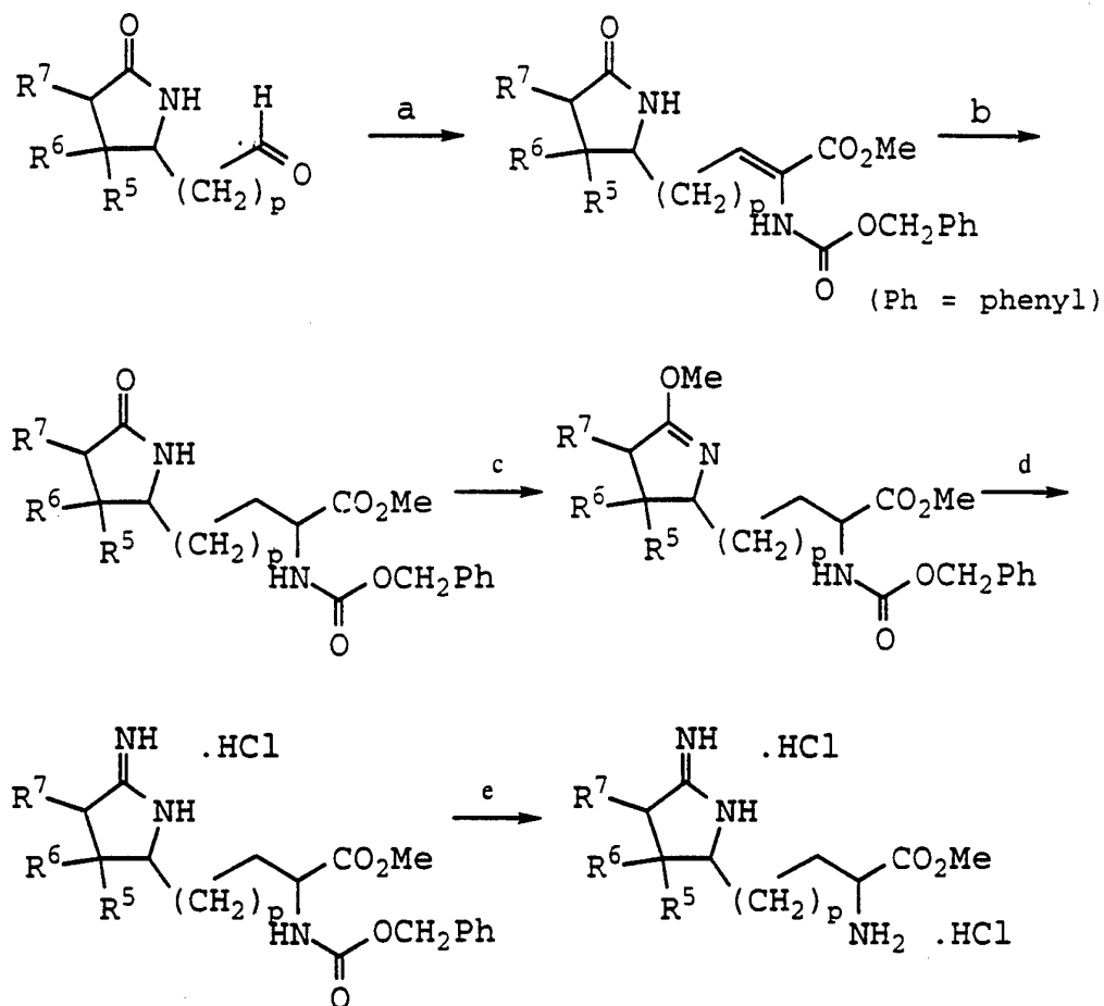
Scheme 5:
