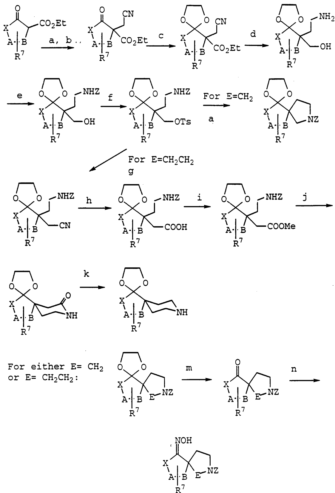
Scheme 9:
