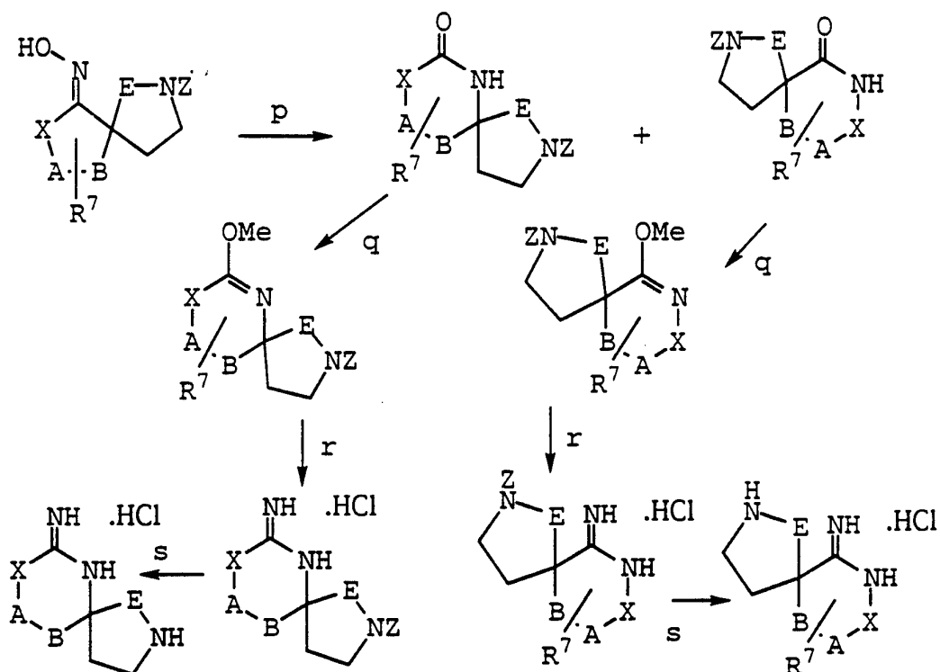
Scheme 9 (continued)
