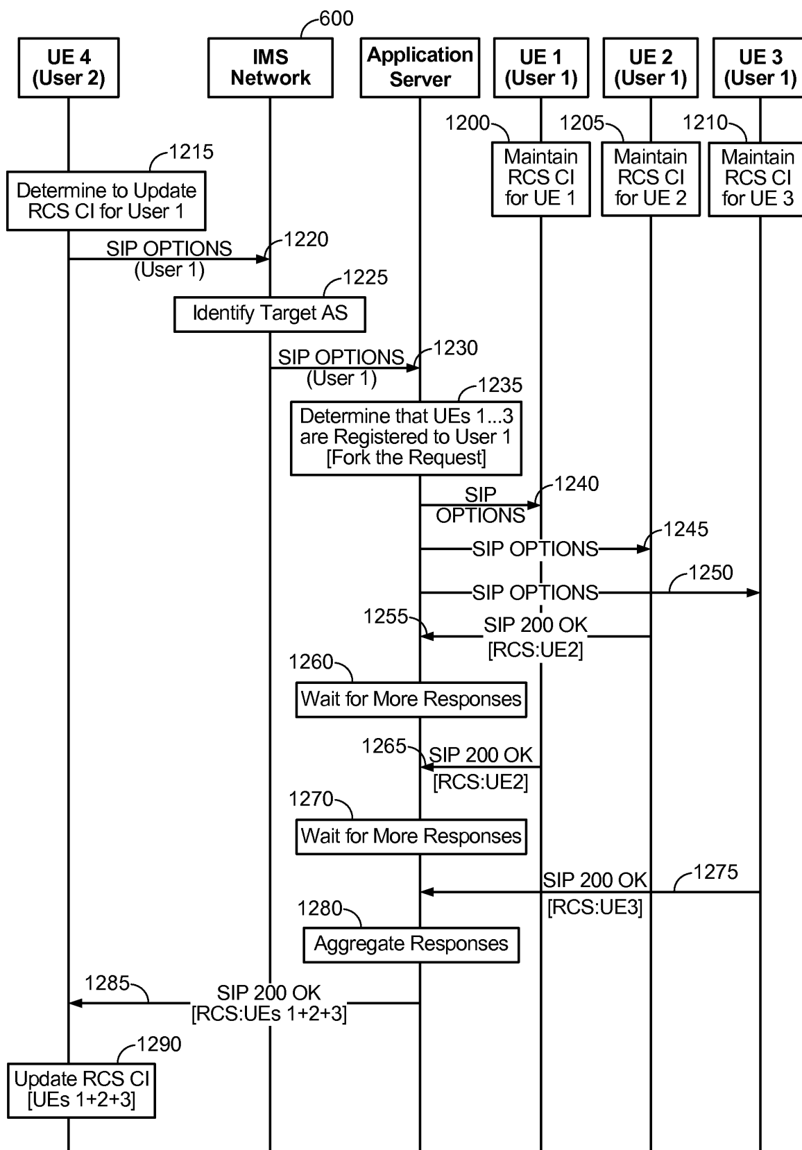
FIG. 12 CONVENTIONAL ART
