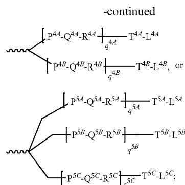
Formula (IV)
