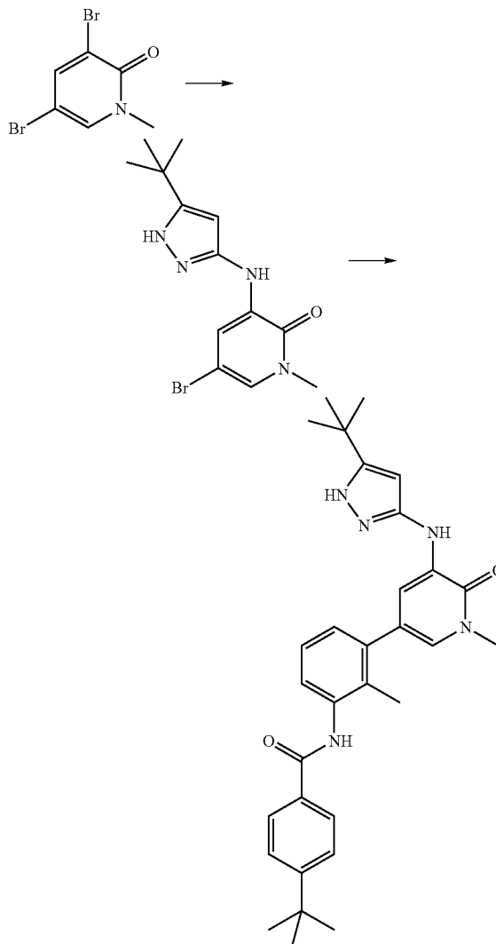
3,5-Dibromo-1-methyl-1H-pyridin-2-one
