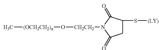
Thioether Linkage
