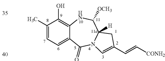
Anthramycin
