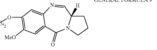
GENERAL FORMULA 9
