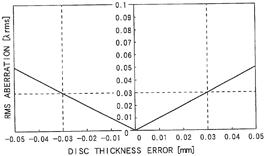
RELATIONSHIP BETWEEN DISC THICKNESS ERROR OF DISC ADAPTED FOR HIGH-VISION (WAVELENGTH: 405nm, NA: 0.85 AND SUBSTRATE REFRACTIVE INDEX: 1.58) AND ABERRATION THEREOF
