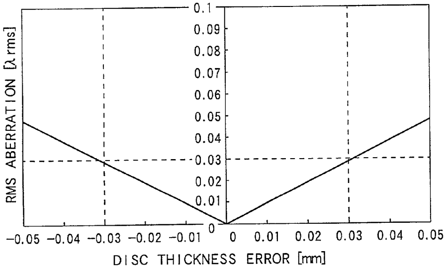
RELATIONSHIP BETWEEN DISC THICKNESS ERROR OF DVD (WAVELENGTH: 650nm, NA: 0.6 AND SUBSTRATE REFRACTIVE INDEX: 1.58) AND ABERRATION THEREOF
