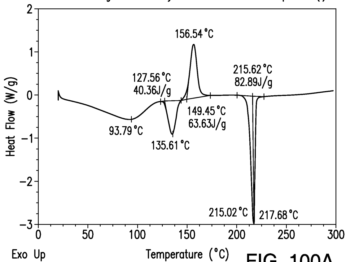
DSC Thermogram of a Hydrate of Racemic Compound (I)
