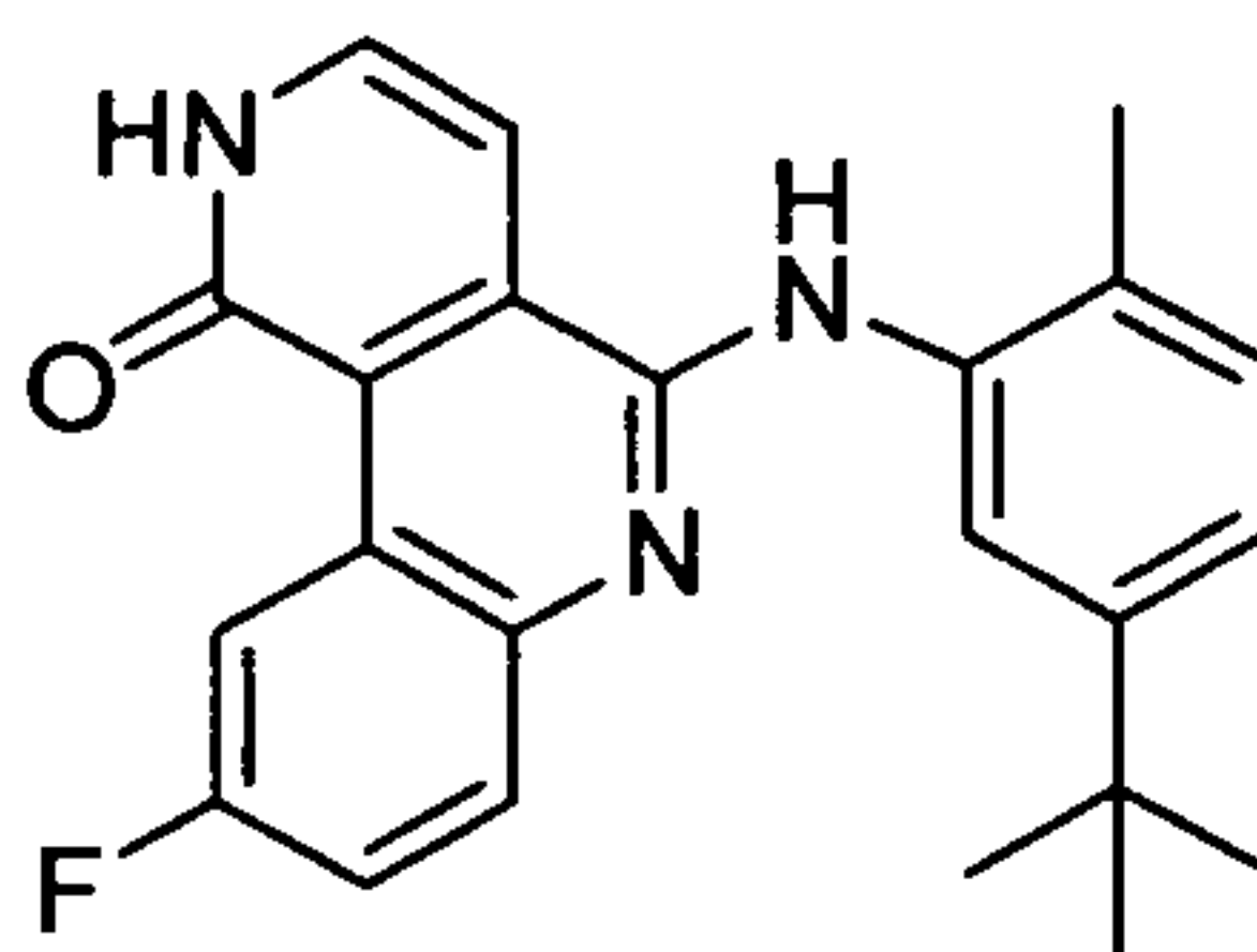
5-[(5- tert -Butyl-2-methylphenyl)amino]-9-fluorobenzo[c]-2,6-naphthyridin-1(2H)-one
