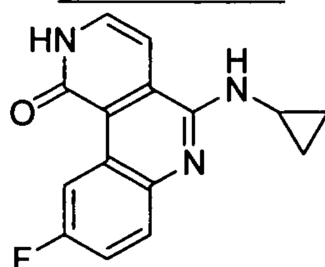
5-(Cyclopropylamino)-9-fluorobenzo[c]-2,6-naphthyridin-1(2H)-one
