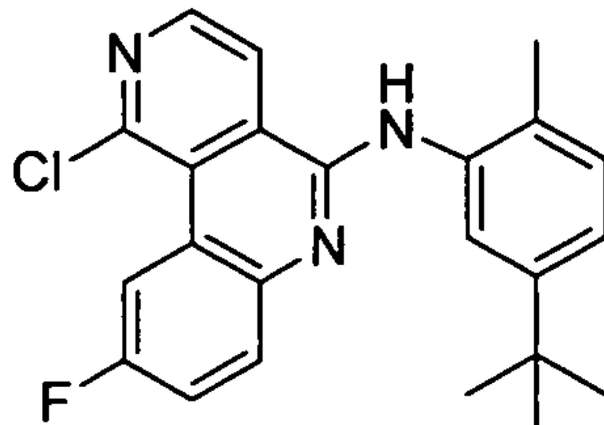
5-[(5- tert -Butyl-2-methylphenyl)amino]-9-fluorobenzo[c]-2,6-naphthyridin-1(2H)-one
