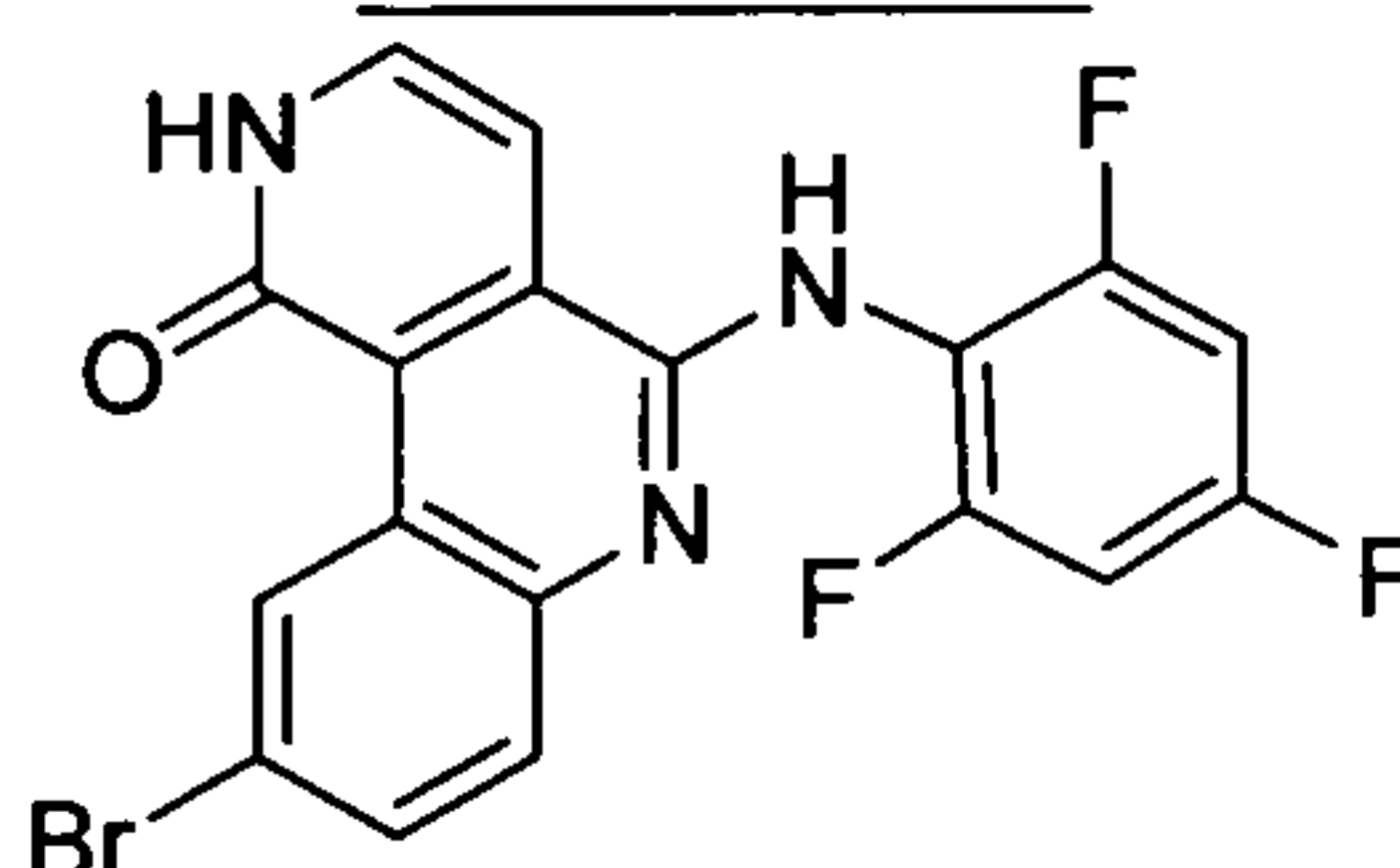
9-Bromo-5-[(2,4,6-trifluorophenyl)amino]benzo[c]-2,6-naphthyridin-1(2H)-one
