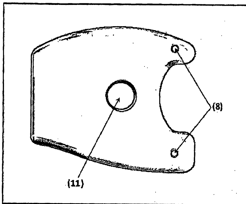
Figure 3-C Tibial Tool, Top View
