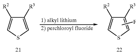
Scheme VII
