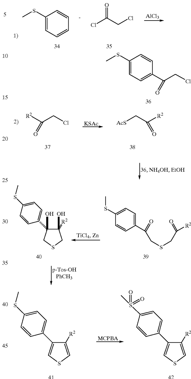
Scheme XIII
