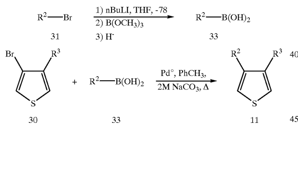
Scheme XII
