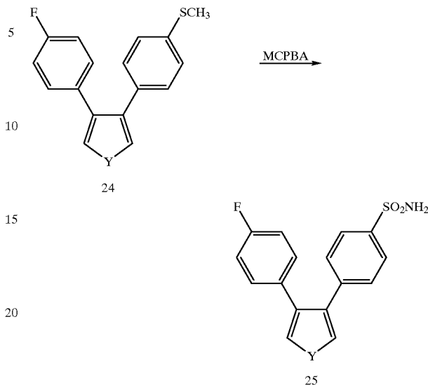
Scheme IX
