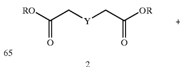
Scheme III
