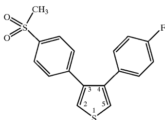
3-(4-Methylsulfonylphenyl)-4-(4-fluorophenyl) thiophene
