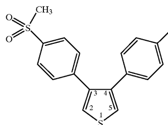
3-(4-Methanesulfonylphenyl)-4-(4-methylphenyl)-thiophene
