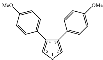
3,4-Bis(4-methoxyphenyl)thiophene
