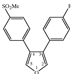
3-(4-Fluorophenyl)-4-(4-methylsulfonylphenyl)furan
