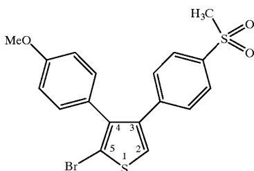
3-(4-Methylsulfonylphenyl)-4-(4-methoxyphenyl)-5-bromothiophene
