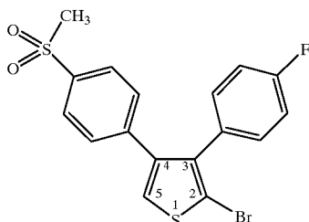
4-(4-Methylsulfonylphenyl)-3-(4-fluorophenyl)-2-bromothiophene
