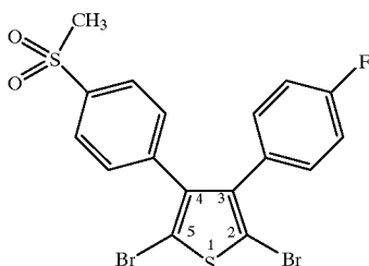
4-(4-Methylsulfonylphenyl)-3-(4-fluorophenyl)-2,5-dibromothiophene
