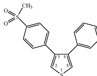
3-(4-Methanesulfonylphenyl)-4-phenyl-thiophene
