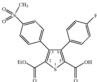
2-Ethoxycarbonyl-4-(4-fluorophenyl)-3-(4-methanesulfonylphenyl)-thienyl-5-carboxylic acid
