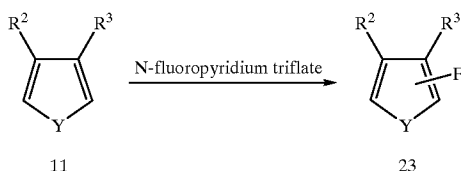
Scheme VIII
