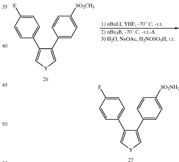
Scheme X
